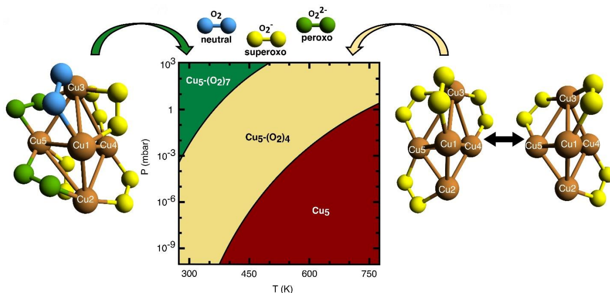
Figure 6. Theoretical characterization of \text{Cu}_5\text{-(O}_2\text{)}_n complexes. Phase diagram, showing the most probable \text{Cu}_5\text{-(O}_2\text{)}_n complexes at each variable pair ( p, T ).
