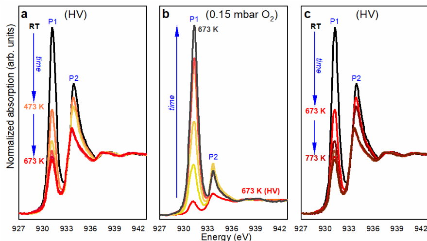
Figure 4. In-situ Cu L_3 -edge XANES spectra of Cu_5/HOPG in low concentration (see text). a, Stage 1, in HV during heating. b, Stage 2: 0.15 mbar of oxygen pressure at 673 K. c, Stage 3: reduction during heating in HV. Each spectrum that is presented corresponds to a condition that was reached after waiting for the spectrum to not change.
