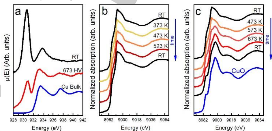
Figure 2. a, Cu L_3 -edge XANES spectra of \text{Cu}_5/\text{HOPG} in high concentration. Spectra were collected in high vacuum at RT (black) and after at 673 K (red). The spectrum of metallic Cu is shown for comparison (blue). b, XANES spectra at the Cu K-edge of \text{Cu}_5/\text{HOPG} with the same concentration as in a, collected in air from RT to 523 K and back to RT. c, XANES spectra at the Cu K-edge of the same sample used in b, collected in air from RT up to 673 K and back to RT. The spectrum of CuO reference (blue) is shown for comparison. Each spectrum that is presented corresponds to a condition that was reached after waiting for the spectrum to not change.
