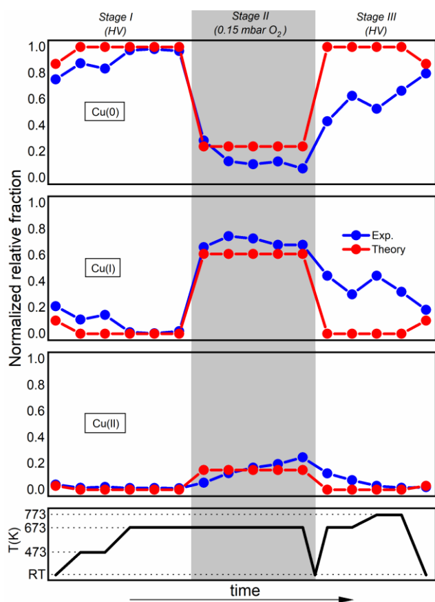
Figure 5. Comparison between theoretically and experimentally determined fractions of Cu(0), Cu(I) and Cu(II) oxidation states in Cu_5/HOPG in HV and 0.15 mbar of O_2 . Theoretical values are determined through a Boltzmann-weighted average of the Helmholtz free energies for each complex and their associated distributions of oxidation states (see SI Section 9). Error bars of experimental points are not shown for simplicity. The time axis is only indicative of the experimental sequence for each condition. Each spectrum used to obtain this figure corresponds to a condition that was reached after waiting for the spectrum to not change.
