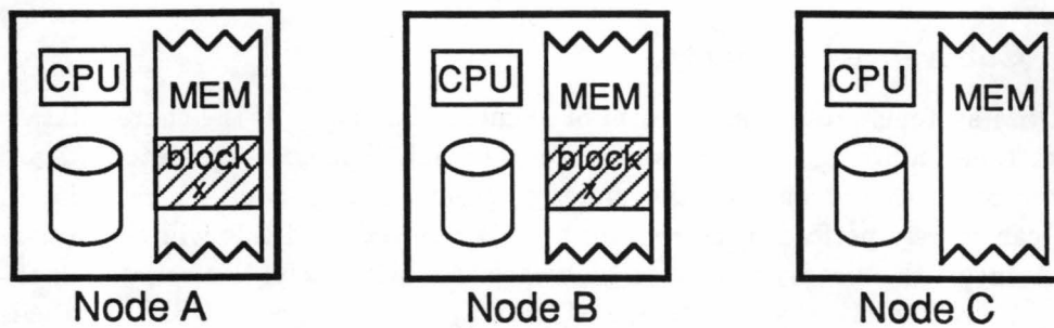
(a) Block x is replicated on Nodes A and B, referenced by Node C
