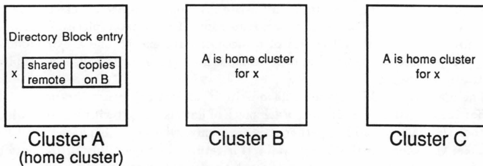
(b) DASH distributed directory-based scheme
