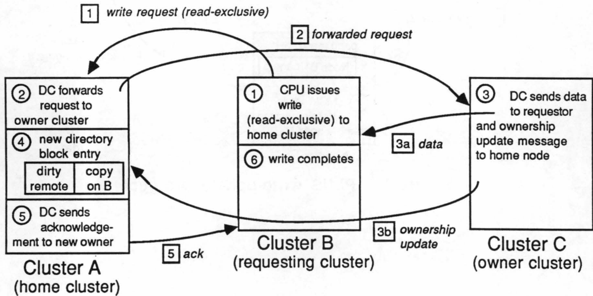
Figure 4: Simplified DASH write-invalidate protocol
