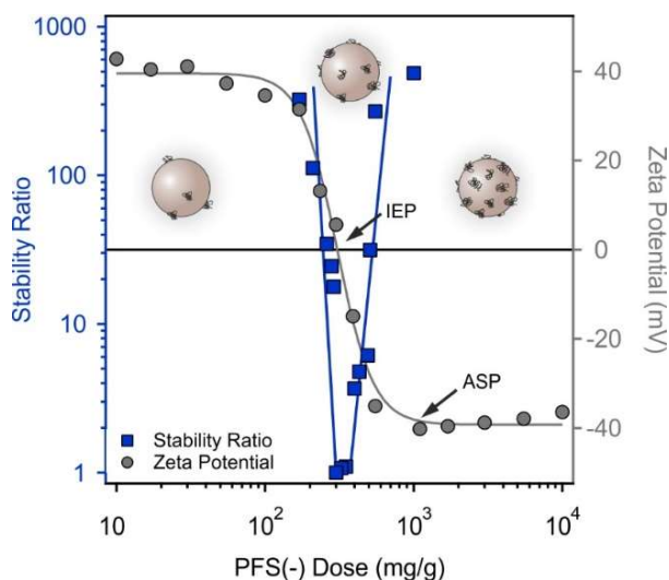
Fig. 2 Adsorption of PFS(-) on AL at pH 4.0 and ionic strength of 1.0 mM. Zeta potential and stability ratio of AL (25 mg/L) at different PFS(-) doses (mg PFS(-)/g AL). The solid lines are eye guides and the graphic insets demonstrate the increased adsorption of PFS(-) at higher doses.
