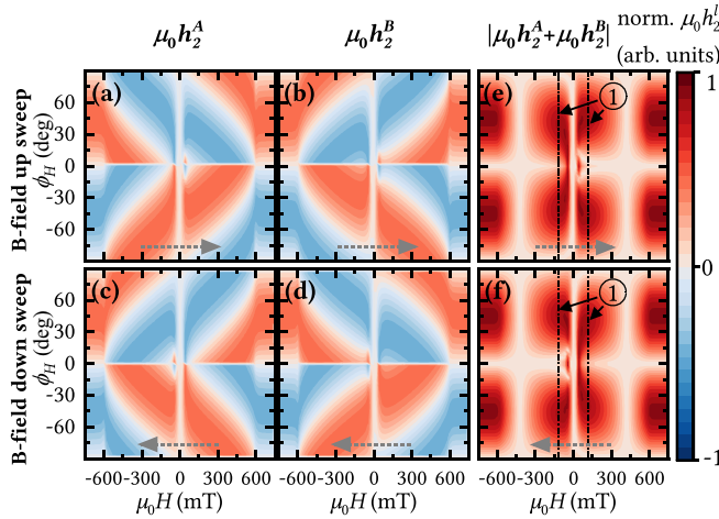
FIG. 7. (a)–(d) The calculated in-plane magnetoacoustic driving field magnitude \mu_0 h_2^l(\mu_0 H, \phi_H) in the bottom (A) and top magnetic layer (B) of the SAF is shown for the magnetic field up and down sweep. For the SAW-SW resonance fields at \mu_0 H \approx \pm 120 mT (Ⓛ), the magnetizations \mathbf{M}^A and \mathbf{M}^B are almost antiparallel aligned to each other. In this configuration, efficient magnetoacoustic excitation of the optical SW mode is possible if |\mu_0 h_2^A + \mu_0 h_2^B| is large. (e) and (f) The sum of the driving fields |\mu_0 h_2^A + \mu_0 h_2^B| shows an asymmetric behavior with respect to \mu_0 H = 0 and differs for the magnetic field up and down sweeps. Thus, the SAW transmission magnitude of resonance Ⓛ depends on the field sweep direction, as observed in Fig. 3. The magnitude of the driving fields was normalized to \max(\mu_0 h_2^A + \mu_0 h_2^B) .
