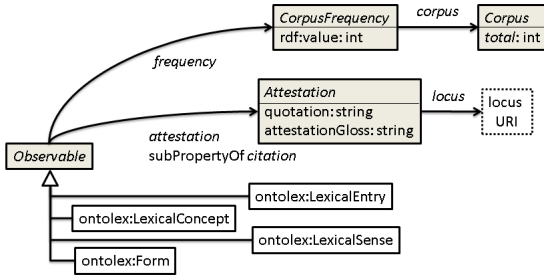
Figure 2: OntoLex-FrAC module structure
