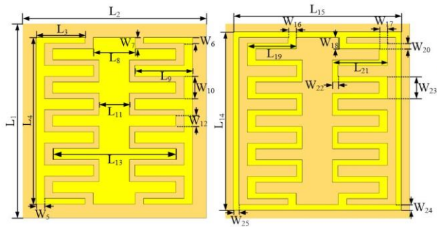
FIGURE 3. The proposed unit cell configuration and parameters.
