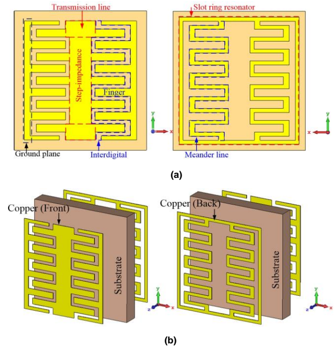
FIGURE 1. The proposed structure of FSS unit cell (a) Front and back structure of FSS unit cell (b) Material layer of FSS unit cell.
