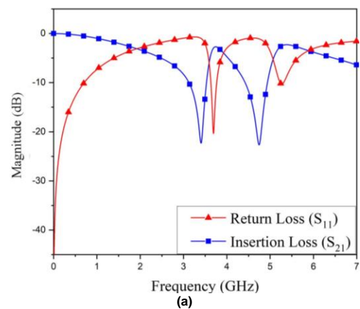
FIGURE 4. The wave transmission test in (a) first case and (b) second case.
