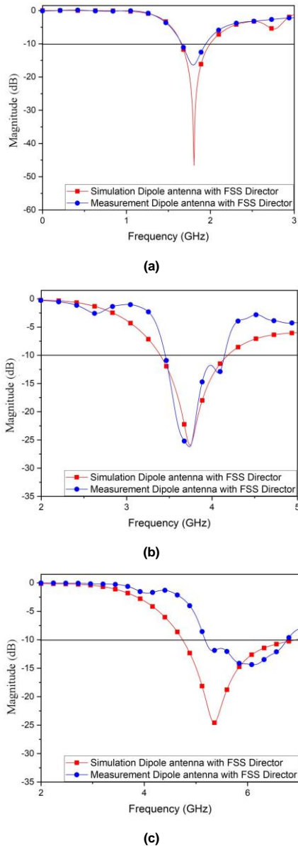
FIGURE 22. The measured reflection coefficient of the antenna with FSS director at the frequency of (a) 1.8 GHz, (b) 3.7 GHz, and (c) 5.2 GHz.
