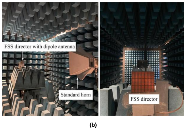
FIGURE 21. The prototype antenna with FSS director (a) configuration and (b) measured in the anechoic chamber room.
