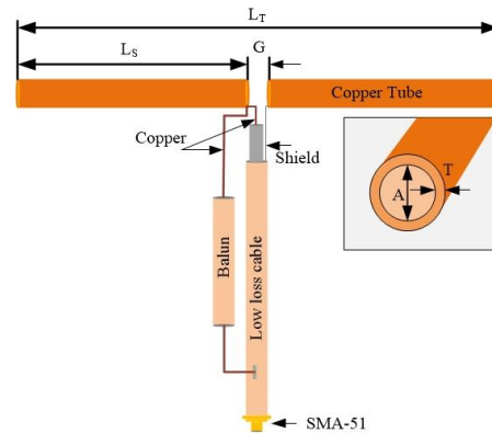
FIGURE 15. The dipole antenna configuration created by copper tube connected to balun and fed by SMA-51.
