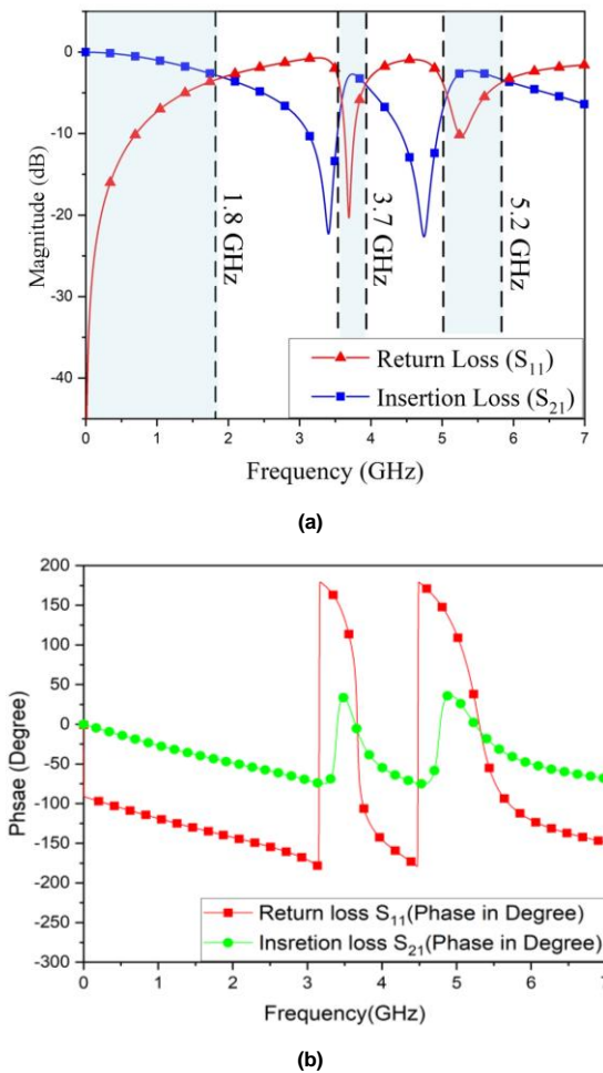
FIGURE 6. The simulation result of proposed FSS unit cell (a) Magnitude of S_{11} and S_{21} and (b) Phase of S_{11} and S_{21} .
