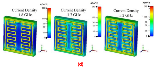
FIGURE 11. The simulation results on the proposed unit cell of (a) the E -field and H -field at front layer, (b) the E -field and H -field at back layer, (c) current distribution with E_x-H_y and E_y-H_x at front layer, and (d) current distribution with E_x-H_y and E_y-H_x at back layer.
