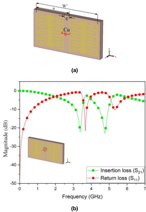
FIGURE 14. The connection between the proposed unit cell (a) configuration (b) simulation result of the |S_{11}| and |S_{21}| .
