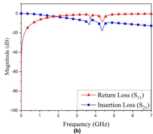
FIGURE 5. The simulation result of S_{11} and S_{21} with (a) PMC on Y-axis and PEC on X-axis and (b) PEC on Y-axis and PMC on X-axis.
