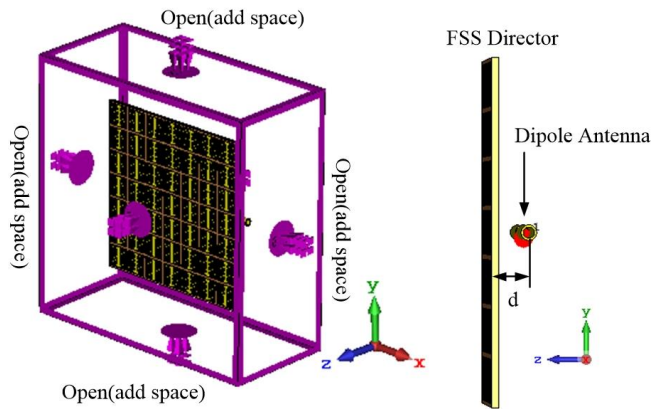
FIGURE 17. The boundary condition configuration of the simulation process for the antenna with the FSS director.
