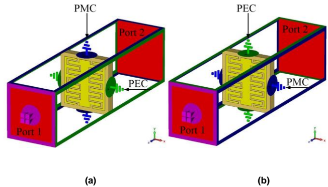
FIGURE 4. The wave transmission test in (a) first case and (b) second case.
