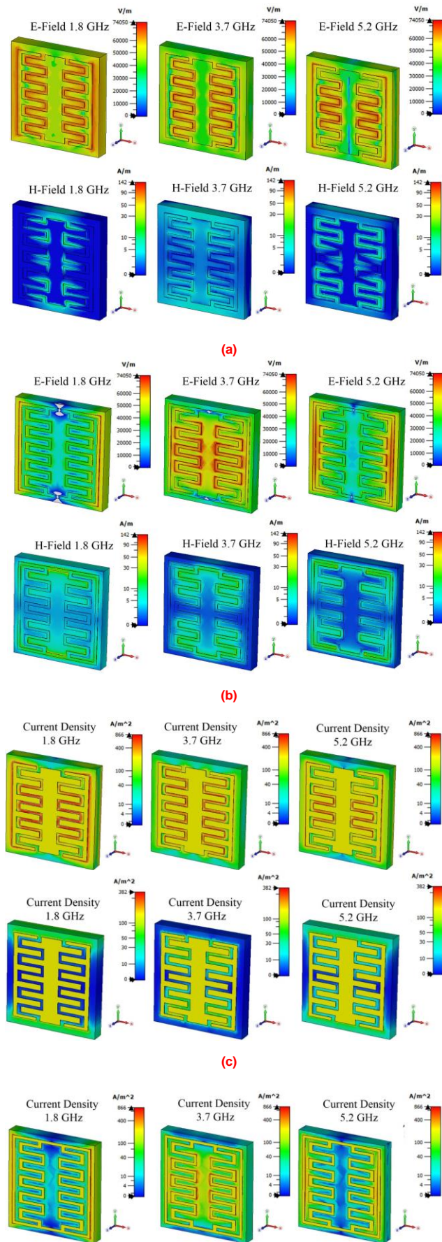
FIGURE 11. The simulation results on the proposed unit cell of (a) the E -field and H -field at front layer, (b) the E -field and H -field at back layer, (c) current distribution with E_x-H_y and E_y-H_x at front layer, and (d) current distribution with E_x-H_y and E_y-H_x at back layer.
