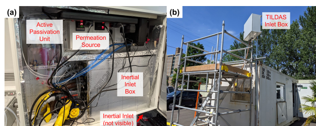
Figure 2. (a) Field configuration for HCl TILDAS inlet system. (b) Mounted inlet system at Manchester field site.
