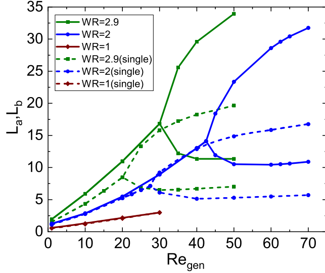
Figure 12: Vortex length against generalised Reynolds in single and multi inlet geometries of the same WR and n = 1 . Lines are provided to guide the eye.
