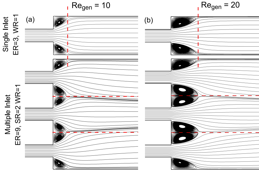
Figure 11: Comparison of the corner vortex size between the single inlet ( ER = 3 , WR = 1 ) and multi inlet geometry E ( SR = 2 , WR = 1 , ER = 9 ) for n = 1 at (a) Re_{gen} = 10 and (b) Re_{gen} = 20 . The horizontal dashed lines demarcate three regions similar in geometry to that of the single inlet and the vertical lines highlight the similarity in corner vortex length.
