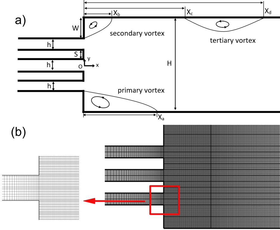
Figure 1: (a) Schematics of the base geometry with three equal inlet channels and one larger outlet channel ( SR = 1 , WR = 2 ) and associated geometric parameters. (b) Mesh near the sudden expansion ( -5 \leq x/h \leq 10 ), with zoomed view near the expansion for improved clarity. The flow is from left to right.
