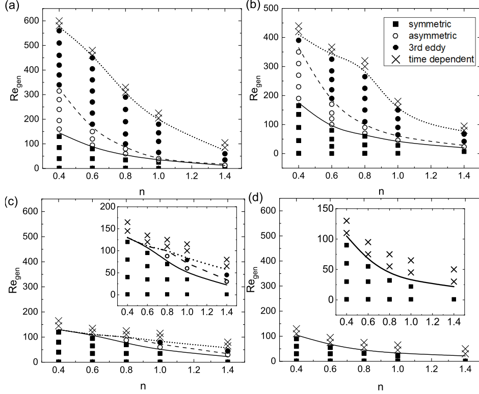
Figure 9: Flow maps in the Re_{gen} - n parameter space investigated for different geometries: (a) geometry A: SR = 0.1 , WR = 2.9 , (b) geometry B: SR = 0.5 , WR = 2.5 , (c) geometry D: SR = 1.5 , WR = 1.5 and (d) geometry E: SR = 2 , WR = 1 . Legend is common to all plots. Lines are provided to guide the eye.
