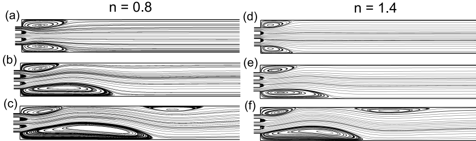
Figure 6: Flow patterns in the (a)(d) symmetric ( Re_{gen} = 0.8Re_{gen,cr1} ), (b)(e) asymmetric ( Re_{gen} = 0.5(Re_{gen,cr1} + Re_{gen,cr2}) ) and (c)(f) 3 rd eddy regime ( Re_{gen} = 1.2Re_{gen,cr2} ), for n = 0.8 (a-c), and n = 1.4 (d-f), for the base geometry ( SR = 1 , WR = 2 ).
