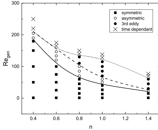
Figure 5: Re_{gen} - n flow map, showing the flow regimes and flow regime transitions present in the investigated range of Re_{gen} and power-law index for the base geometry ( SR = 1 , WR = 2 ). Lines are provided to guide the eye.
