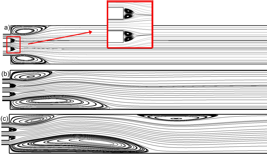
Figure 3: Flow patterns in the (a) symmetric regime ( Re_{gen} = 0.8Re_{gen,cr1} ) with insert to highlight the intermediate vortices, (b) asymmetric regime ( Re_{gen} = 0.5(Re_{gen,cr1} + Re_{gen,cr2}) ) and (c) 3 rd eddy regime ( Re_{gen} = 1.2Re_{gen,cr2} ), for a Newtonian fluid ( n = 1 ) in the base geometry ( SR = 1 , WR = 2 ).
