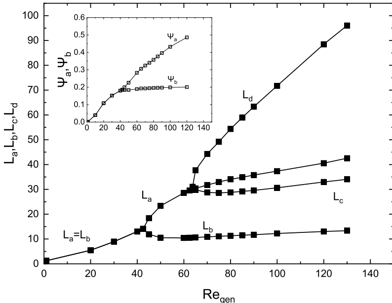
Figure 4: Non-dimensional vortex length ( L_R ) variation against generalised Reynolds number for a Newtonian fluid ( n = 1 ) in the base geometry ( SR = 1 , WR = 2 ). The inset shows the normalised corner vortex intensity ( \Psi_R ) as a function of Re_{gen} for the same case.
