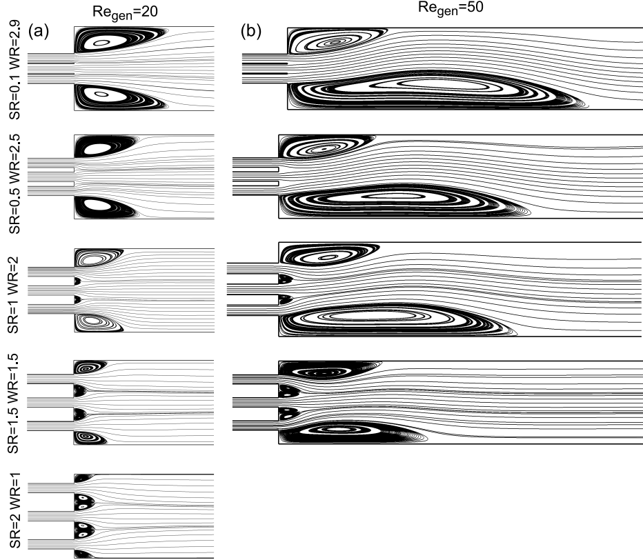
Figure 8: Newtonian fluid flow patterns in the symmetric regime, (a) Re_{gen} = 20 , and the asymmetric regime, (b) Re_{gen} = 50 , for all geometries. Note that geometry E ( SR = 2 , WR = 1 ) does not exhibit a steady asymmetric regime.
