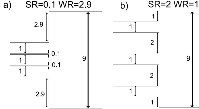
Figure 2: Diagrams of geometry (a) A and (b) E showing the relevant normalised widths to highlight the differences as SR and WR are changed over the range of spacings.
