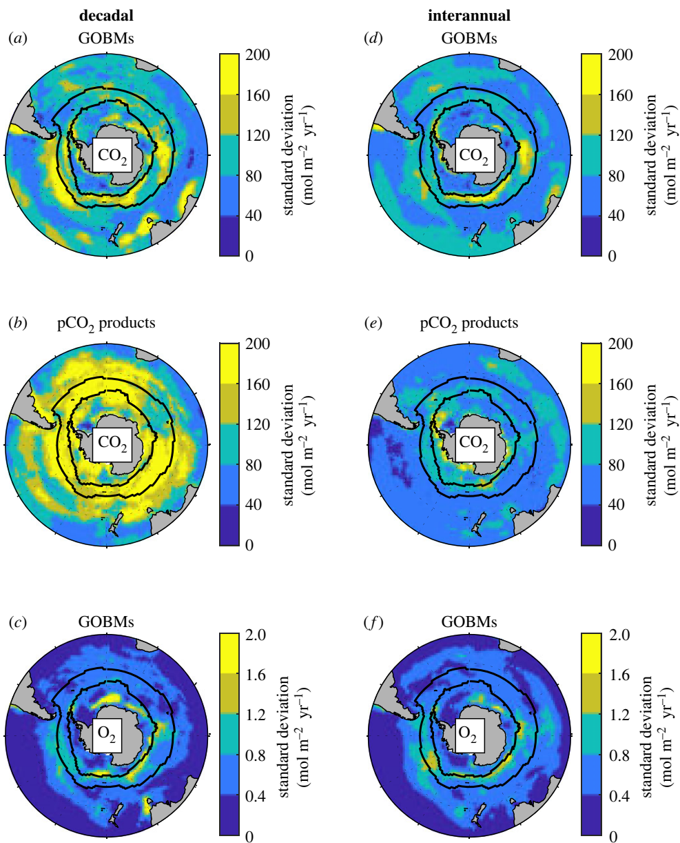
Figure 3. Standard deviation of the decadal (left) and interannual (right) variability of \text{CO}_2 and \text{O}_2 air–sea fluxes. For \text{CO}_2 (a,b and d,e), the averaged maps from GOBMs and from \text{pCO}_2 products are shown, while for \text{O}_2 (c and f) only GOBMs could be used to study the spatial patterns. Note the differences in units and colour scales between \text{O}_2 and \text{CO}_2 maps. The black lines represent the average location of the Subantarctic Front (northern line) and of the September extent of sea ice (southern line). Maps from individual GOBM and \text{pCO}_2 product are available in the electronic supplementary material (figures S1–S6). (Online version in colour.)
