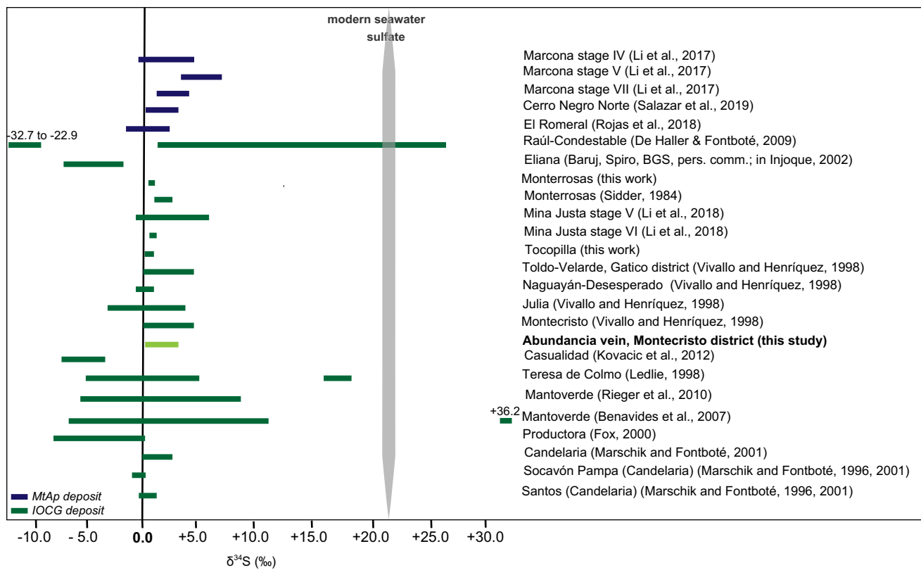
Fig. 9 \delta^{34}\text{S} compositions for MtAp and IOCG deposits in Chile and Peru
