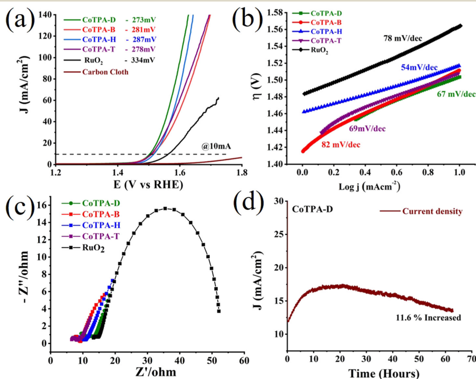
Fig. 7 (a) OER polarization curves (scan rate 1 \text{ mV s}^{-1} ), (b) Tafel slopes, (c) electrochemical impedance spectra of CoTPA MOFs and (d) chronoamperometric studies of CoTPA-D.
