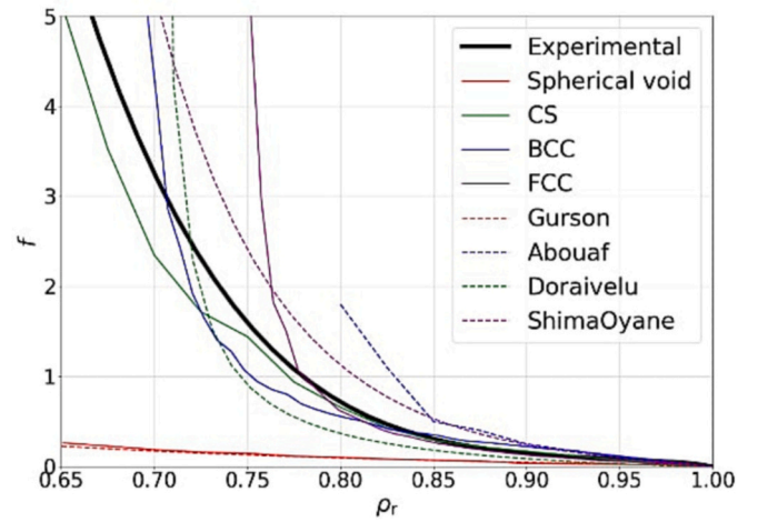
Fig. 5.. Correlation obtained in [25] among experimental results, numerical results from FEM and bibliography results. Abbreviations for configurations: CS (Cubic Simple), BCC (Body Centered Cubic) and FCC (Face Centered Cubic).
