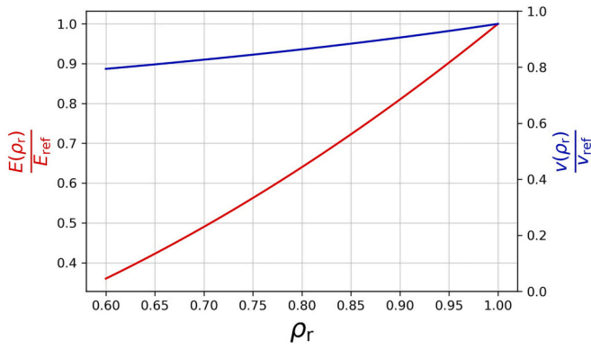
Fig. 2.. Evolution of elastic modulus (red) and Poisson's modulus (blue) for different relative density levels.
