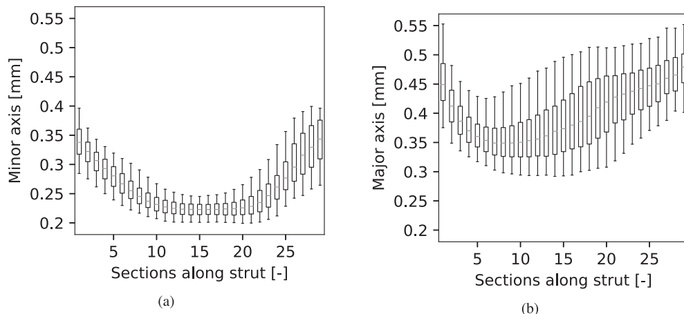
Fig. 11. Distribution of the (a) minor axis and (b) major axis of the elliptical cross-section along the strut axis.
