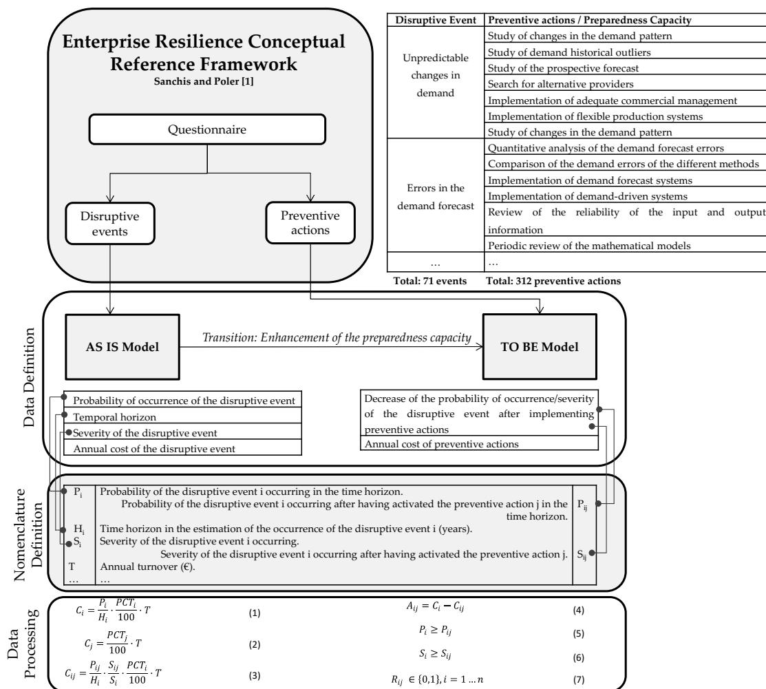
Figure 2. Data-modelling approach.
