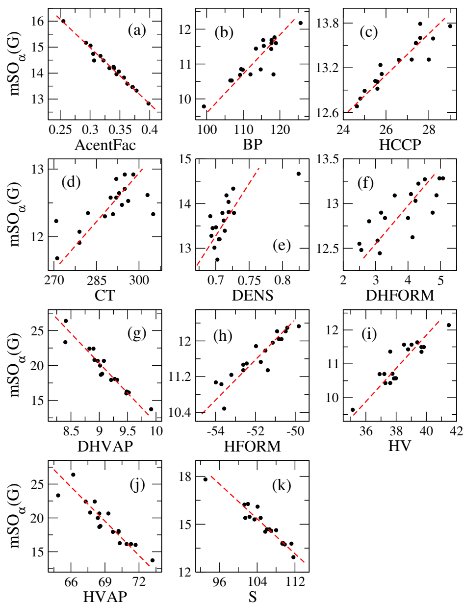
Figure 1: Mean Sombor index mSO_\alpha(G) vs. the physicochemical properties of octane isomers, for the values of \alpha that maximize the correlations: (a) \alpha = 0 , (b) \alpha = -8.19 , (c) \alpha = -0.87 , (d) \alpha = -2.05 , (e) \alpha = -0.53 , (f) \alpha = -1.28 , (g) \alpha \rightarrow \infty , (h) \alpha = -4.23 , (i) \alpha \rightarrow -\infty , (j) \alpha \rightarrow \infty , and (k) \alpha = 0.58 . Red dashed lines are the linear QSPR models of Equation (5), with the regression and statistical parameters resumed in Table 3.
