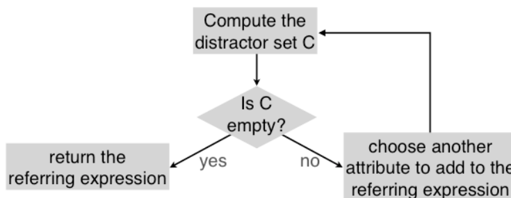
Fig. 2: The traditional REG model.
