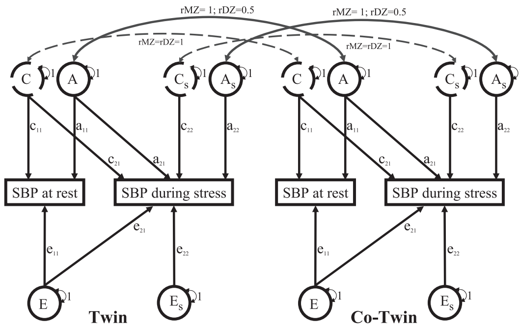
Figure 2. Bivariate twin model for genetic and environmental influences on systolic blood pressure (SBP). Biometrical genetic theory specifies that the additive genetic factors (denoted by A and As) of (monozygotic) MZ twins are perfectly correlated (1.0), whereas those of dizygotic (DZ) twins are correlated 0.5. Common environmental factors shared by twins from the same family (denoted by C and Cs) are correlated unity for both types of twins, whereas the unique environmental influences (E and Es) are always uncorrelated. Path coefficient a_{11} quantifies the effect of genetic influence A on SBP at rest, a_{21} quantifies the effect of A on SBP during stress, and a_{22} quantifies the effect of emergent genes in As on SBP during stress. In a similar way, path coefficients e_{11} , c_{11} , e_{21} , and c_{21} quantify the effects of common and unique environmental influences E and C on SBP at rest and during stress. e_{22} and c_{22} quantify the effect of emergent environmental influences in Es and Cs on SBP during stress.
