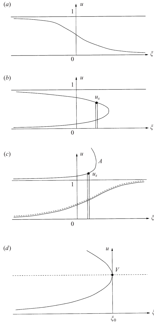
FIGURE 11. Travelling wave solutions: (a) M_w < 1, V = \gamma ; (b) 1 < M_w < \sqrt{2\gamma/(\gamma-1)}, V = \gamma ; (c) \sqrt{2\gamma/(\gamma-1)} < M_w, V = \gamma ; (d) M_0 = \sqrt{2\gamma/[(\gamma-1)V^2]} .
