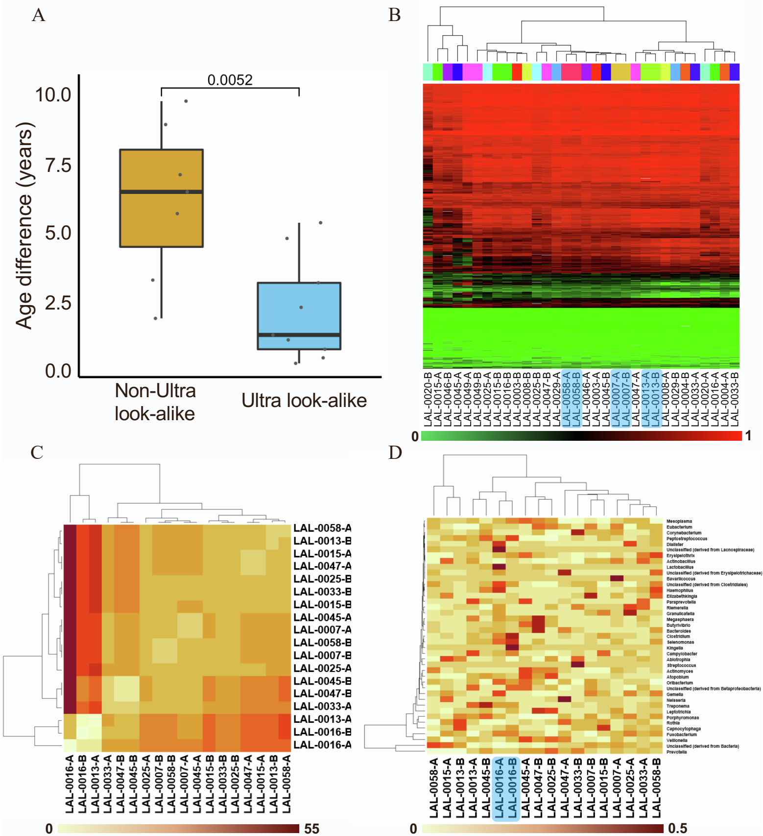
Figure S6. DNA methylation age estimation, mEQTLs and microbiome analyses. Related to Figure 3. A. DNA methylation age estimation using the Hannum method for the 16 look-alike couples. Intrapair age estimation differences are significantly smaller (two-sided Mann-Whitney-Wilcoxon test P-value = 0.0052) among the 9 “ultra” look-alike pairs compared to the non-ultra look-alike pairs. B. Heatmap shows supervised genome-wide DNA methylation hierarchical clustering with bootstrap of the 16 look-alikes, using the 1,379 methylation \beta -values obtained from MethylationEPIC array after selecting all those CpGs located within a window of 100 base pairs from any of the 19,277 SNP’s found to be shared in all “ultra” look-alike pairs. Colors represent a continuous quantification of methylation beta values at each CpG site where green highlights unmethylated CpG’s (0), black, 50% methylated CpG’s (0.5) and red, fully methylated CpG’s (1). Clustered “ultra” look-alikes are shown in a blue rectangle. C, D. Microbiome analysis of the 9 ultra” look-alikes. Heatmaps shows the distances from differences in pair-wise bacterial counts of species found in the microbiome of each look-alike pair (variation in alpha diversity scores) of counts from 0 – 55 ( C ) and relative proportions of the taxonomic profiles at the genus level ( D ) for each sample calculated on a scale of 0 - 0.5. Only the most represented genera are shown. Meta-genomic clustering of each look-alike sample was constructed using Euclidean distances and Ward.D2 hierarchical cluster method. Blue rectangle represents look-alike pairs whose microbiome is more closely related.
