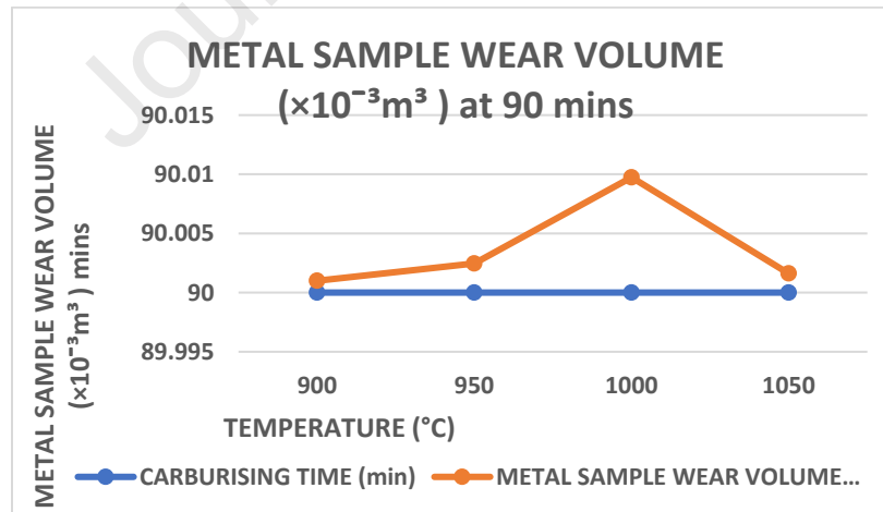
Figure 20: Carburising temperature dependence on wear volume at 90mins
