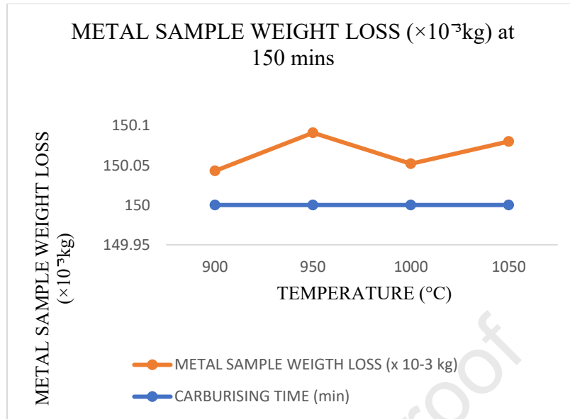
Figure 19: Carburising temperature dependence of metal sample (crushing tool) weight loss at 150mins
