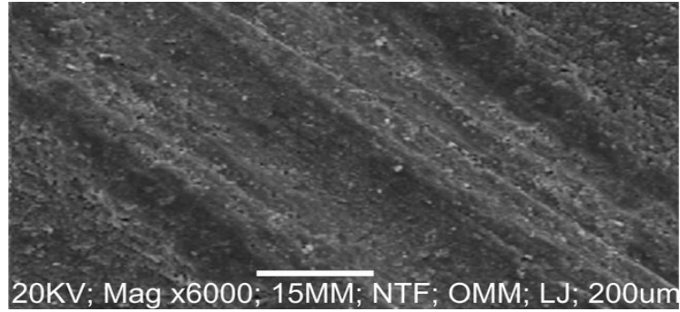
Figure 6: Micrograph showing the surface morphology of the as-received medium carbon steel sample (control)
