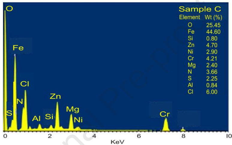
Figure 7: Energy Dispersive Spectroscopy of the elements of the as-received medium carbon steel sample (control)
