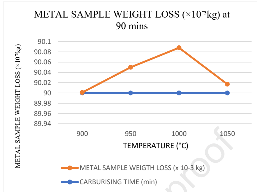
Figure 17: Carburising temperature dependence of metal sample (crushing tool) weight loss at 90mins
