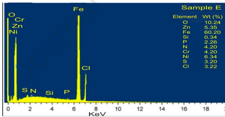
Figure 5: Energy Dispersive Spectroscopy of the elements of the as-received failed mild steel sample
