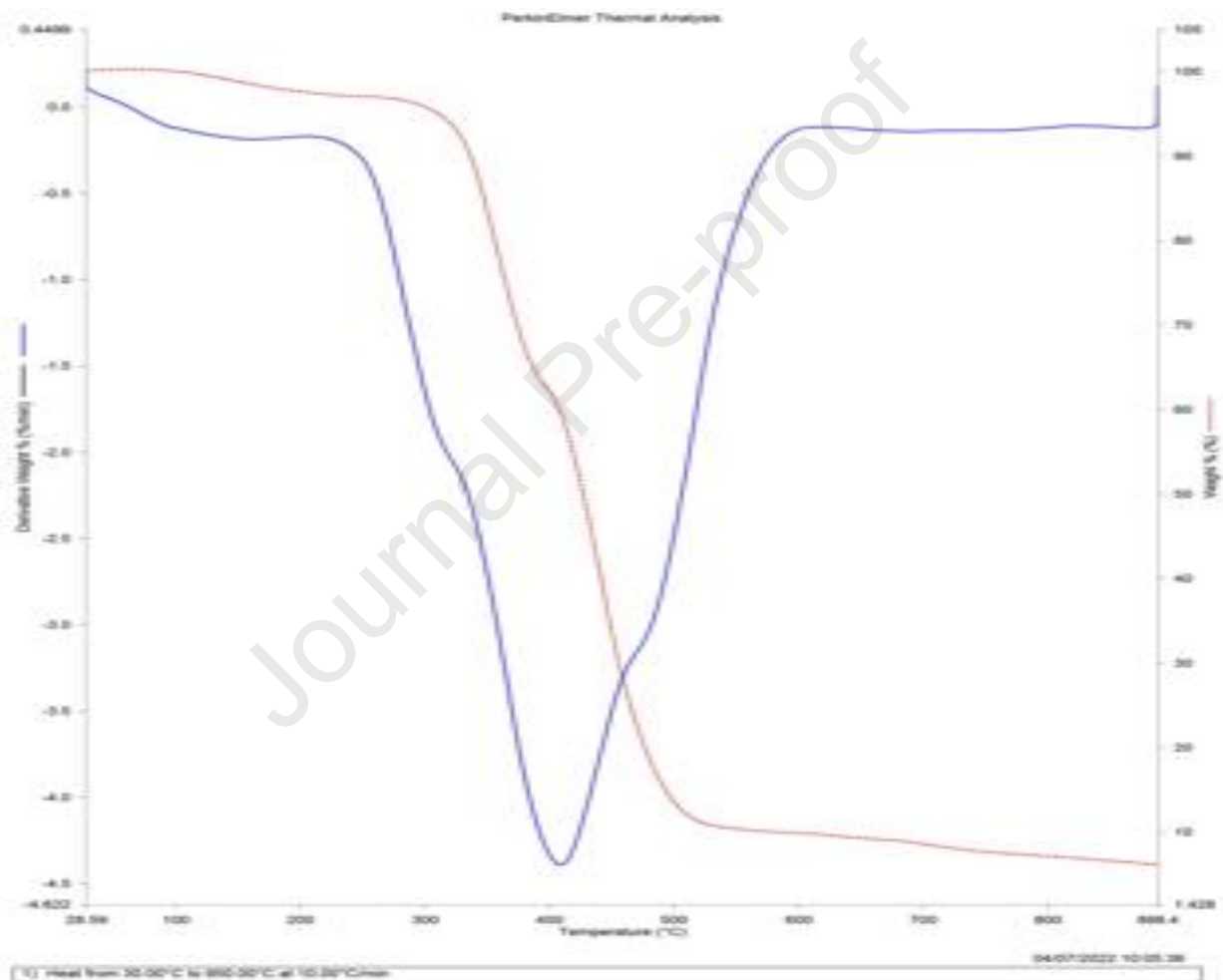
Figure 23: TGA/DTA Curve of samples carburised with palm kernel shell at 1050 °C and 180 mins
