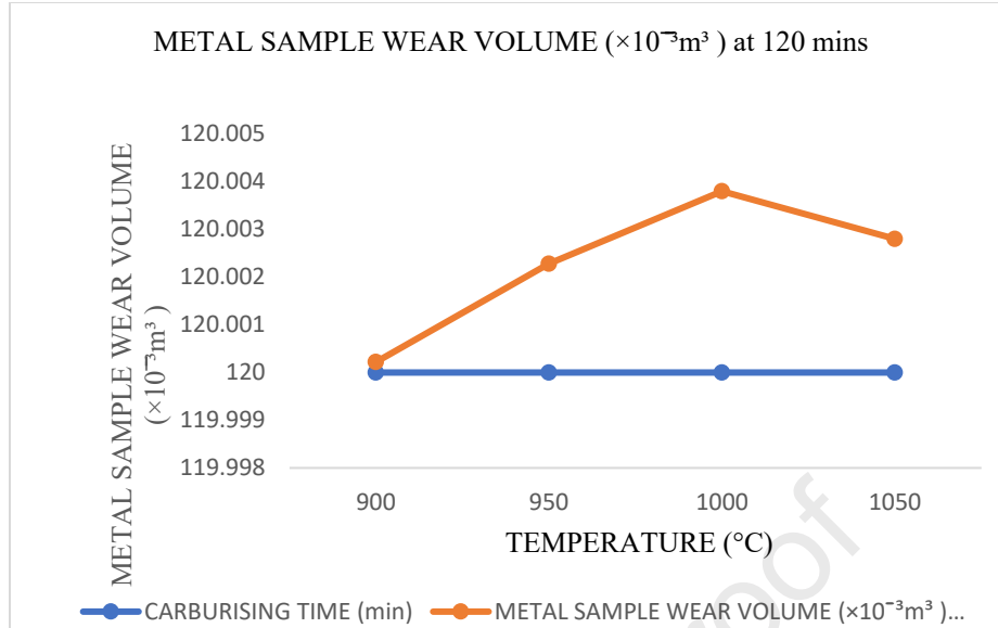
Figure 21: Carburising temperature dependence on wear volume at 120mins
