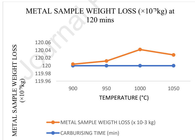
Figure 18: Carburising temperature dependence of metal sample (crushing tool) weight loss at 120mins
