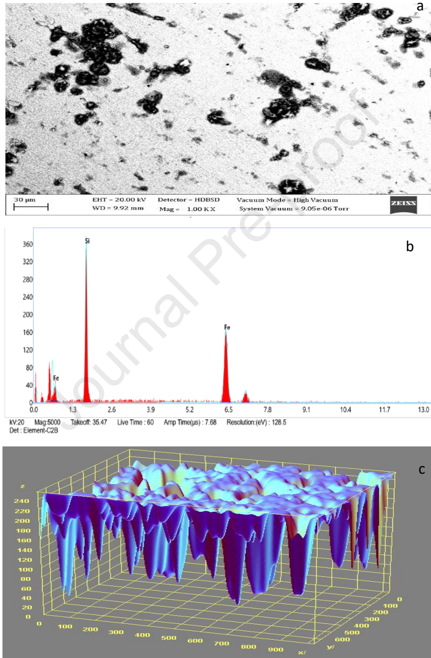
Figure 13: a. Micrograph of medium carbon steel carburised with palm kernel shell at 1000 °C for 3 hr. b. Energy Dispersive Spectroscopy of the elements c. 3D image of the transmission electron microstructural feature of the steel sample
