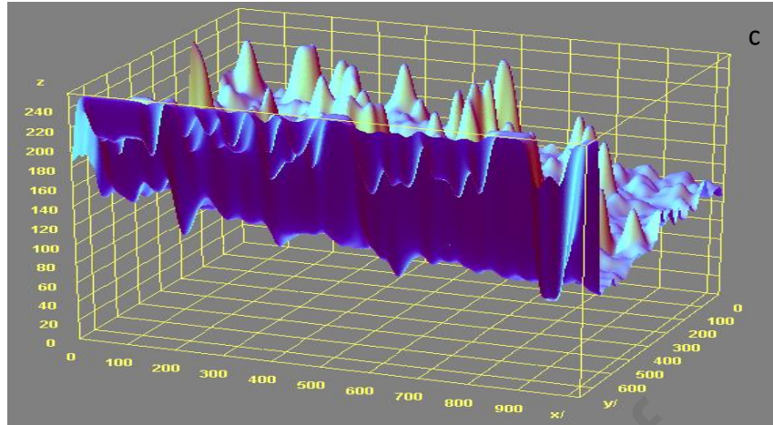
Figure 10: a. Micrograph of medium carbon steel carburised with sawdust, coconut shell, and palm kernel shell at 900 °C for 1 hr b. Energy Dispersive Spectroscopy of the elements c. 3D image of the transmission electron microstructural feature of the steel sample carburised
