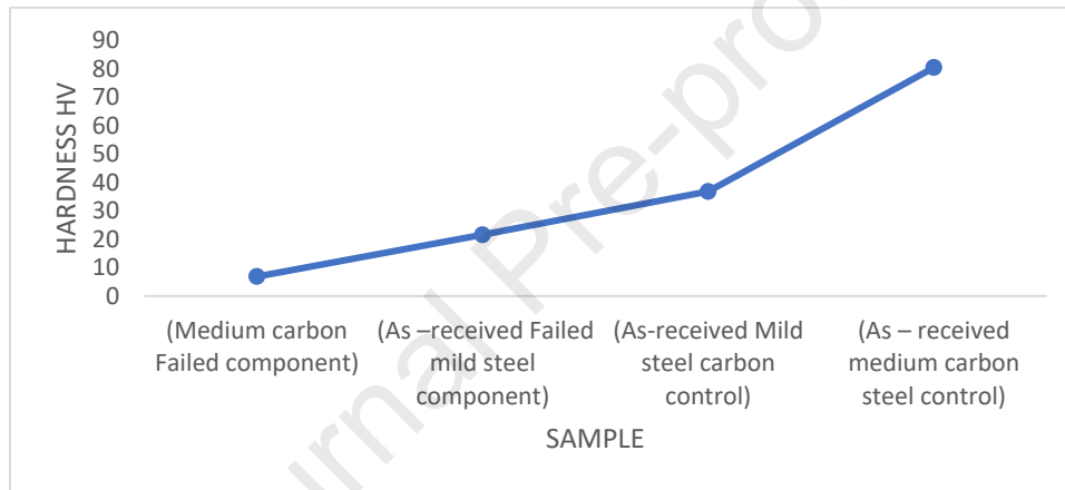
Figure 15: Hardness values of as-received samples
