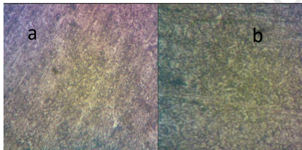
Figure 1: Optical microstructural feature of as-received medium carbon steel (a) (un-failed) (b) carburised
