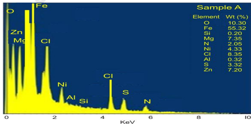
Figure 3: Energy Dispersive Spectroscopy of the elements in failed medium carbon steel sample
