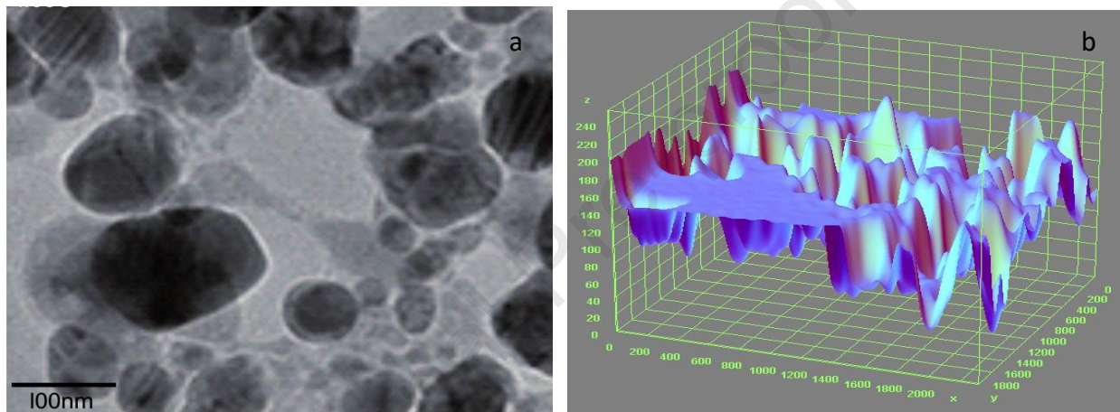
Figure 14: a. TEM Micrograph of the steel sample carburised with palm kernel shell at 1050 °C for 3 hr b. 3D surface plot image of the transmission electron microstructural feature of the steel sample carburised
