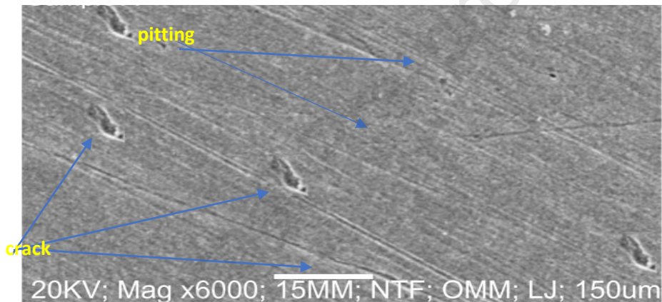
Figure 2: Micrograph showing the surface morphology of as-received failed medium carbon steel sample
