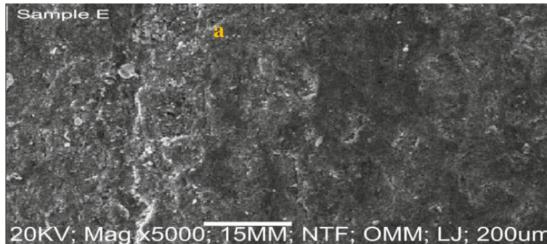
Figure 4: Micrograph showing the surface morphology of the as-received failed mild steel sample
