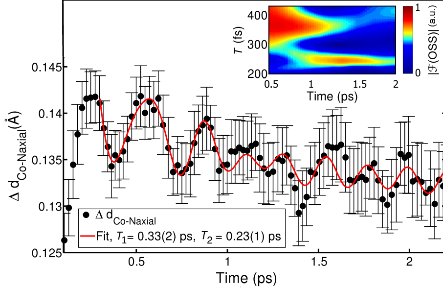
Figure 3. Time evolution of the Co-N bond lengths (black dots) upon photoexcitation, smoothed with 4-point ( \sim 100 fs) moving average filter. The insert shows a time-resolved Fourier transform of the oscillatory part of the difference scattering signal (Fig. 2(a) and Fig. S6 [31]), indicating sequential activation of two vibrational modes. The red line shows a heuristic fit, incorporating sequential activation of first a T_1 \sim 0.33 ps mode and then a T_2 \sim 0.23 ps mode identified as, respectively, breathing- and pincerlike by direct comparison with our DFT calculations.
