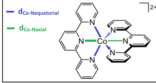
Figure 1. Schematic representation of the structure of [\text{Co}(\text{terpy})_2]^{2+} . The LS \rightarrow HS transition can be induced by photoexcitation with a 530 nm laser pulse and is characterized by an anisotropic expansion of the metal-ligand bonds. Axial and equatorial Co-N bonds are highlighted in different colors.
