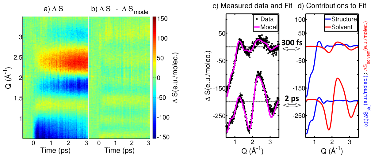
Figure 2. (a) Measured difference scattering signal ( \Delta S ) of photoexcited [\text{Co}(\text{terpy})_2]^{2+} in water. (b) Residuals obtained by subtracting the model ( \Delta S_{\text{model}} ) from the experimental data. (c),(d) Fit of the 1D difference scattering curves at 300 fs and 2 ps. (c) The modelled difference signal (the magenta line) overlaid over the experimental data (black points). (d) The contributions to the model from the structural changes (solute and cage, the blue line) and from the bulk solvent (the red line).
