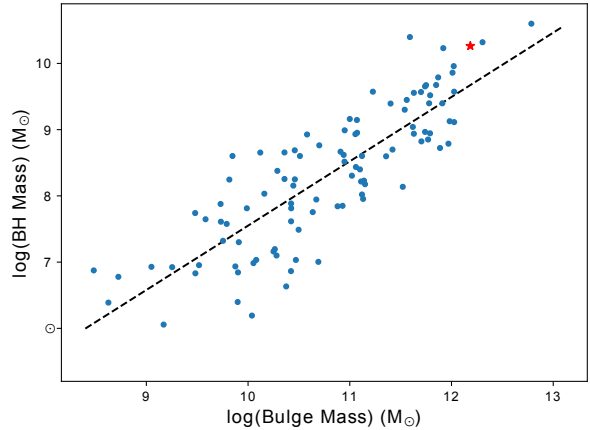
Figure 4. The galaxy sample of Saglia et al. (2016) in the black hole mass vs. galaxy stellar mass diagram (blue points), while the position of OJ 287 is given as a red star. OJ 287 is taken to be 0.3 magnitudes fainter than NGC 4889. Three recent additional measurements have been added: NGC 1600 ( Thomas et al. 2016 ), Abell 1201 central galaxy ( Smith et al. 2017 ) and Holm 15A ( Mehrgan et al. 2019 ). We note that OJ 287 lies within the one sigma scatter from the mean linear correlation (dashed line).
