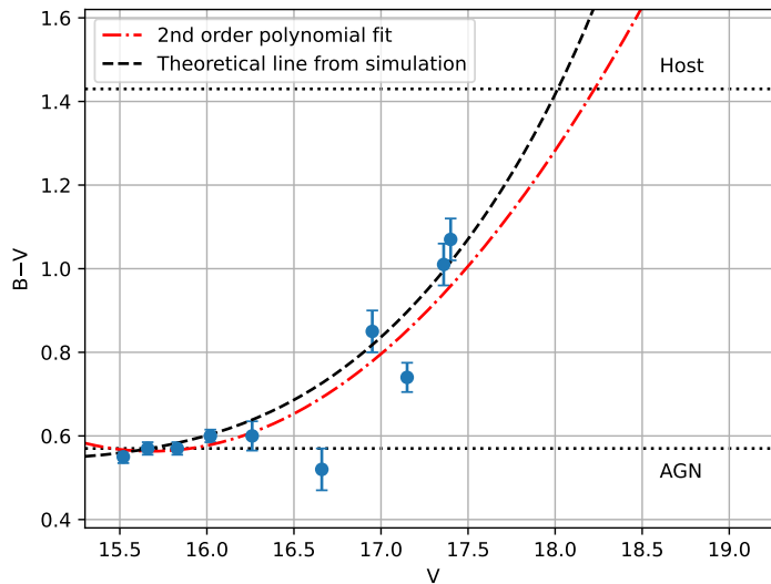
Figure 3. The variation of the B-V colour as a function of V-band magnitude in OJ 287. The points above V=16.2 refer to the 1989 fade, the others come from our Tables 1 and 2, and are averages of ten measurements each. The red dash-dotted line represents a second order polynomial fit to the data points. The black dashed line shows the expected colour index variation if a host of V=18.0 is added to the AGN of constant colour. The horizontal dotted lines represent the expected host galaxy colour and the AGN colour, respectively.
