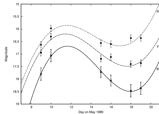
Figure 1. The observations of the 1989 fade of OJ 287 with the Nordic Optical Telescope and the Jacobus Kapteyn Telescope at La Palma, with 2\sigma errorbars. Here we plot the magnitudes in three filters B, V and R. The lines are fifth order polynomial fits through the data points.
