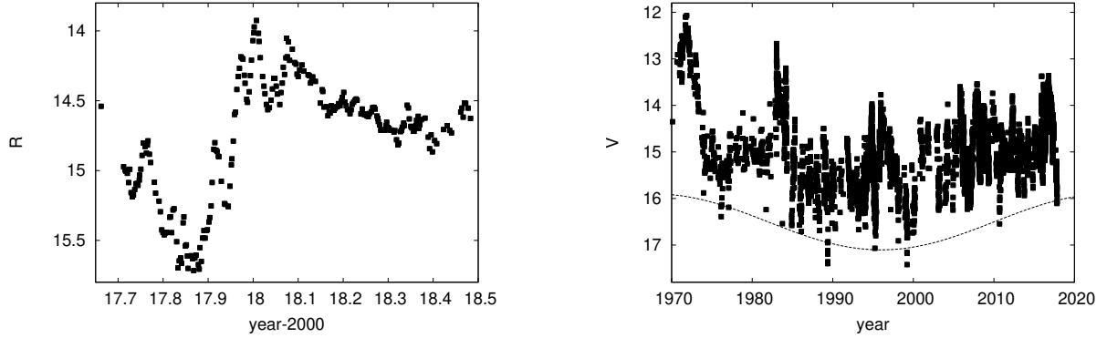
Figure 2. Left panel: The R-band optical light curve of OJ 287 in the 2017/18 season. Right panel: The V-band optical light curve of OJ 287 from 1970 to 2018. The dotted line runs 1.75 magnitudes below the historical mean brightness of OJ 287.
