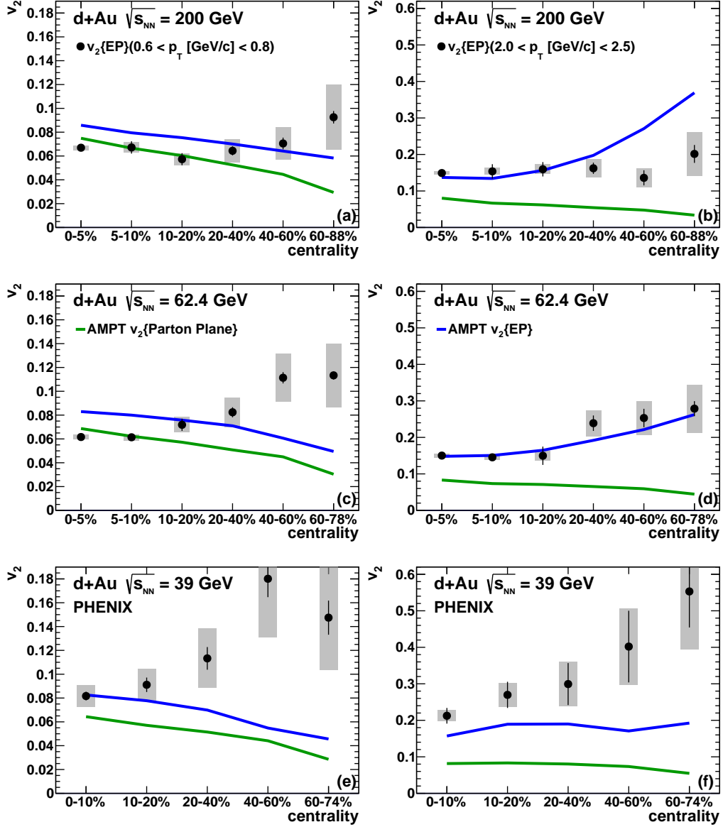
FIG. 10. The value of v_2 as a function of centrality (a,c,e) at 0.6 < p_T [\text{GeV}/c] < 0.8 and (b,d,f) at 2.0 < p_T [\text{GeV}/c] < 2.5 in d+\text{Au} collisions at \sqrt{s_{NN}} = (a,b) 200, (c,d) 62.4, and (e,f) 39 GeV. The upper [blue] curves show calculations from the AMPT model [23] where the v_2 is calculated using the event plane method as described in the text. The lower [green] curves show AMPT calculations where the v_2 is calculated relative to the parton plane.
