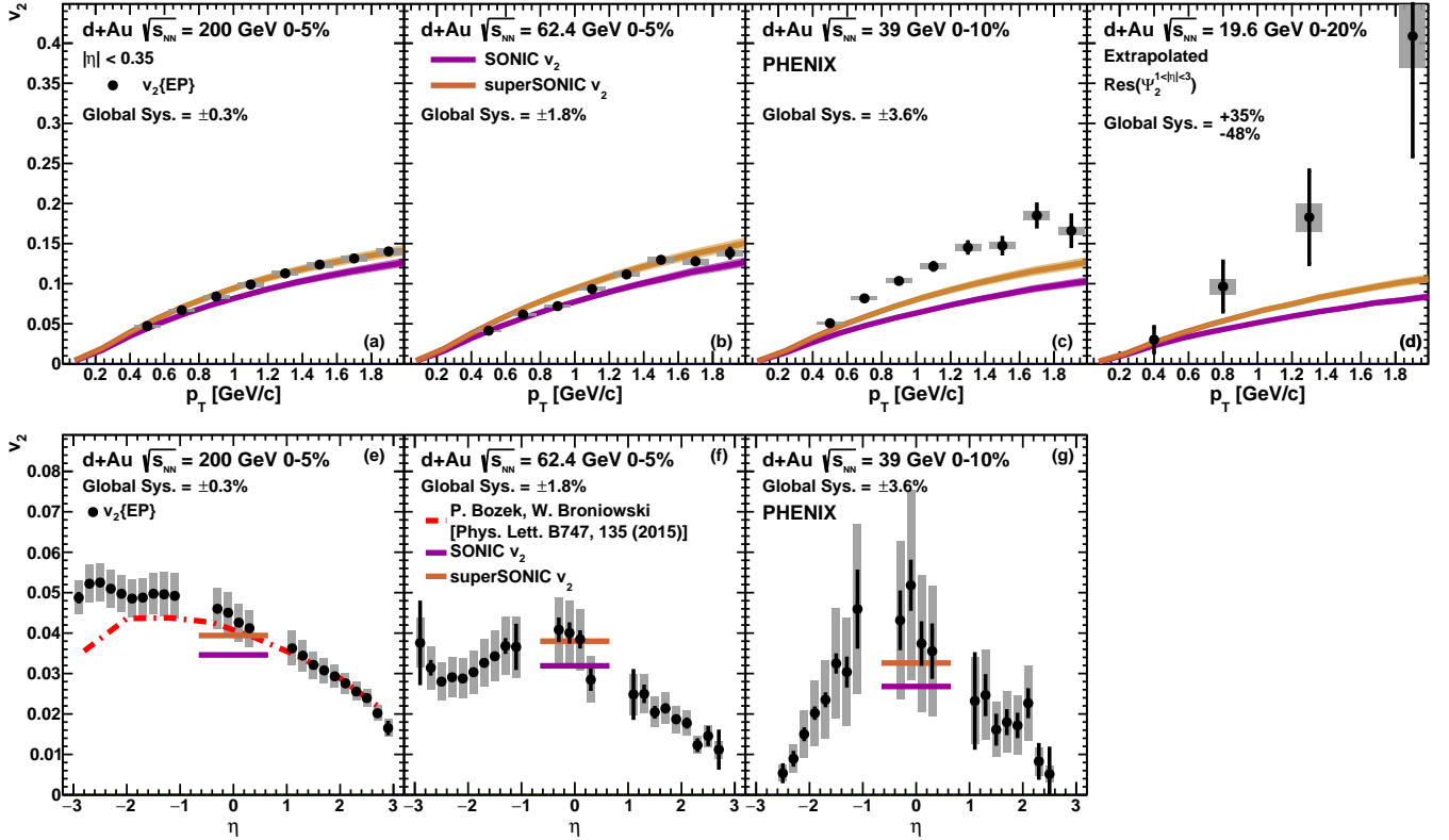
FIG. 11. The value of v_2 as a function of p_T in central d+Au collisions at \sqrt{s_{NN}} = (a) 200, (b) 62.4, (c) 39, and (d) 19.6 GeV. v_2 as a function of \eta in central d+Au collisions at \sqrt{s_{NN}} = (e) 200, (f) 62.4, and (g) 39 GeV. At midrapidity, the [lower] purple and upper [orange] curves show theoretical calculations from SONIC and superSONIC [39], respectively. The dashed [red] curve in panel (e) shows hydrodynamic predictions from Ref. [40].
