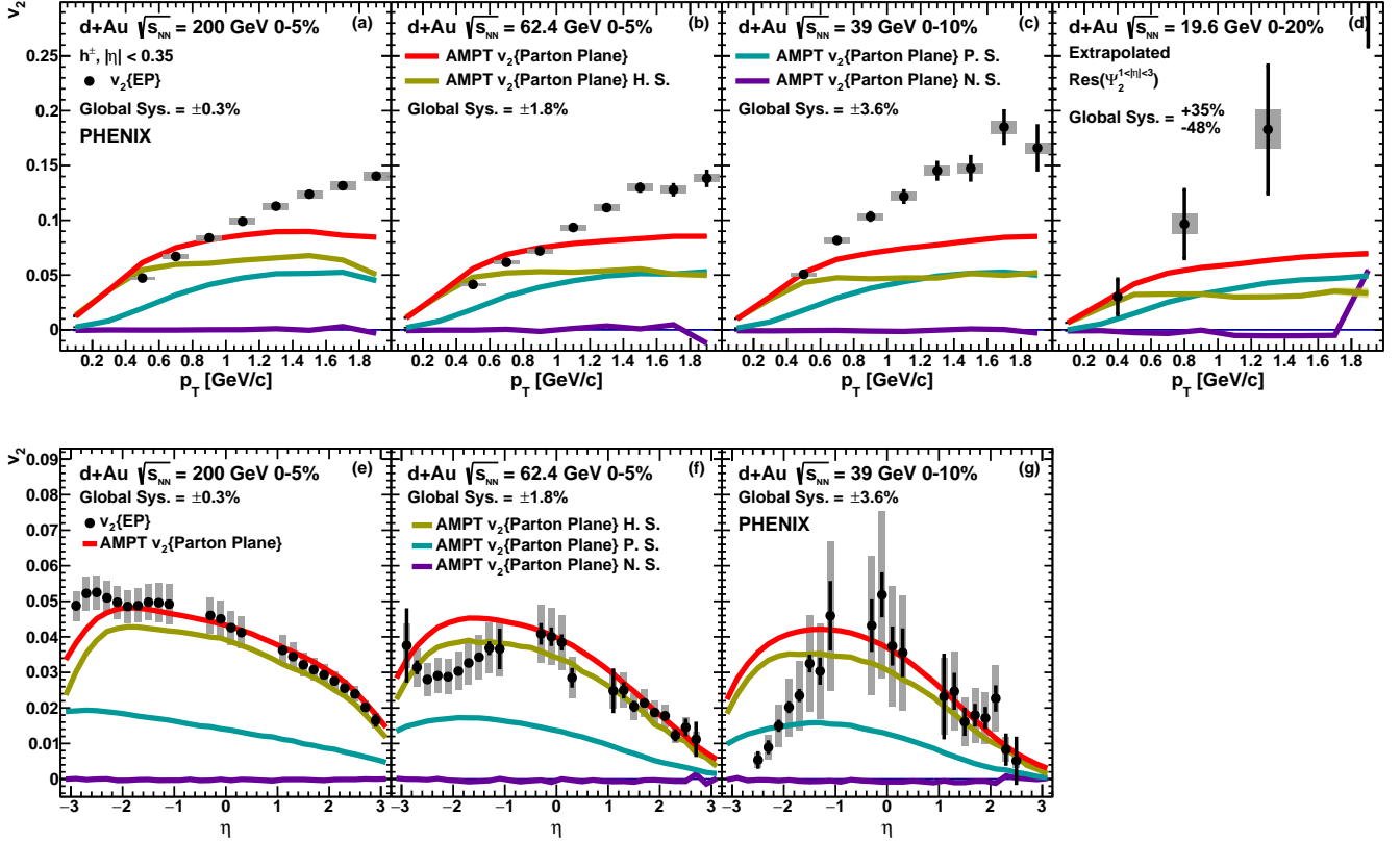
FIG. 17. (a, b, c, d) the value of v_2 vs p_T in central d+Au collisions at \sqrt{s_{NN}} = 200, 62.4, 39, and 19.6 GeV. (e, f, g) the value of v_2 vs \eta in central d+Au collisions at \sqrt{s_{NN}} = 200, 62.4, and 39 GeV. The curves are calculations from AMPT under different conditions. With ordering of curves from top to bottom (a, b, c, d) at p_T = 0.6 and (e, f, g) at \eta = 0 , the uppermost [red] curve is AMPT with both partonic and hadronic scattering; the upper-middle [yellow] curve is AMPT with hadronic scattering only (H.S.); the lower-middle [cyan] curve is AMPT with partonic scattering only (P.S.); and the lowest [purple] curve is AMPT with no scattering (N.S.). For all AMPT curves, the v_2 is calculated relative to the initial parton plane.
