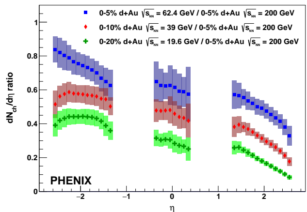
FIG. 7. Ratio of dN_{ch}/d\eta vs \eta in central d +Au collisions at \sqrt{s_{NN}} = 62.4, 39, and 19.6 GeV relative to 0%–5% central d +Au collisions at \sqrt{s_{NN}} = 200 GeV. Systematic uncertainties are shown as filled boxes surrounding each point.
