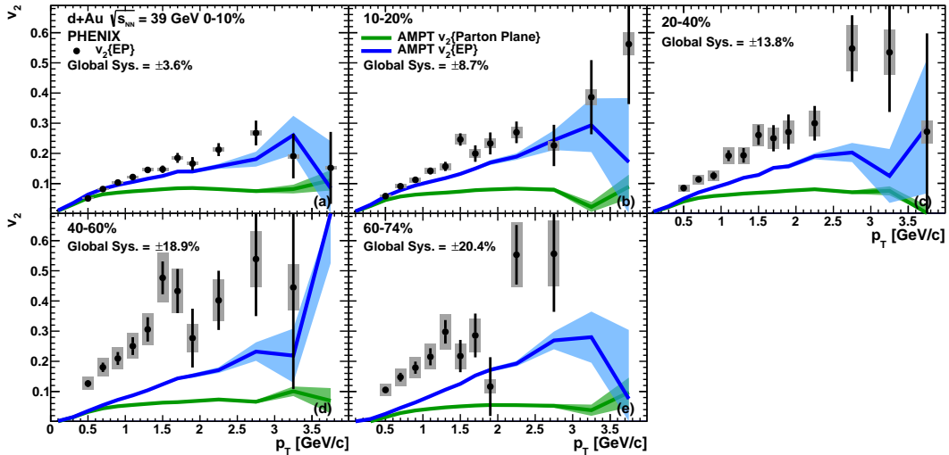
FIG. 16. For d+Au collisions at \sqrt{s_{NN}} = 39 GeV, descriptions of the symbols and curves are the same as in Fig. 14.
