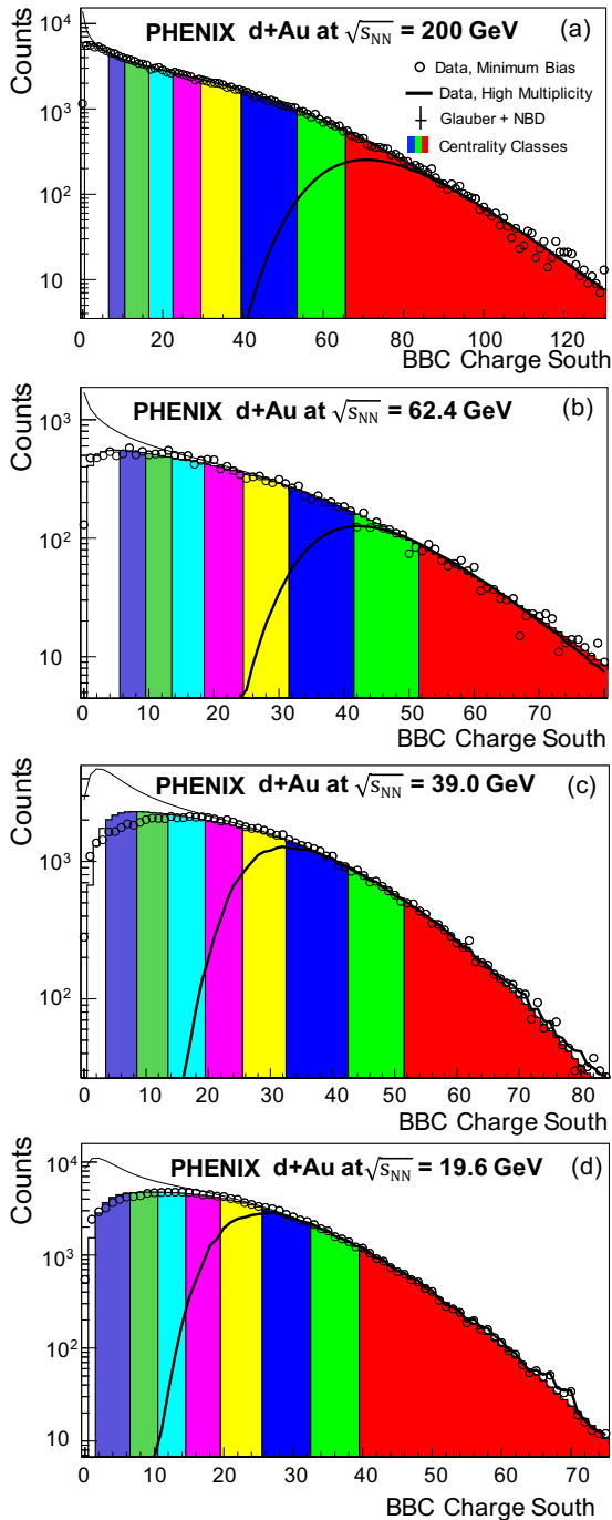
FIG. 2. The distributions of total charge in the BBCS for d+Au collisions at \sqrt{s_{NN}} = 200 (a), 62.4 (b), 39 (c), and 19.6 (d) GeV. The data is from MB collisions, and we note that, as discussed in the text, the MB trigger definition changes with energy. The colored bands represent, from right to left, the centrality categorizations 0%–5%, 5%–10%, 10%–15%, 15%–20%, 20%–30%, 30%–40%, 40%–50%, 50%–60%, and 60%–XX%, where XX is the value of the MB trigger efficiency for each energy, given in Table I. The thick solid line shows the high-multiplicity trigger selection, scaled down to match the MB distribution.
