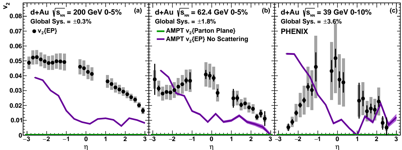
FIG. 9. The value of v_2 as a function of \eta in central d+Au collisions at \sqrt{s_{NN}} = 200, 62.4, and 39 GeV compared to calculations from the AMPT model [23] in which both the partonic and hadronic scatterings have been turned off. The upper [purple] curves show calculations from the AMPT model using the event-plane method as described in the text. The lower [green] curves ( v_2 = 0 in all cases) show calculations from AMPT where v_2 is calculated relative to the parton plane.
