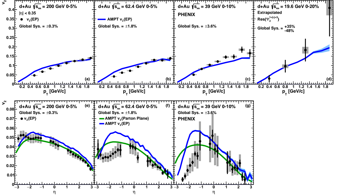
FIG. 8. The value of v_2 as a function of p_T in central d+Au collisions at \sqrt{s_{NN}} = 200 (a), 62.4 (b), 39 (c), and 19.6 (d) GeV. v_2 as a function of \eta in central d+Au collisions at \sqrt{s_{NN}} = 200 (e), 62.4 (f), and 39 (g) GeV. The lower [green] curves show calculations from the AMPT model [23] where the v_2 is calculated relative to the parton plane. The upper [blue] curves show calculations from the AMPT model, where the v_2 is calculated using the event-plane method, as described in the text.
