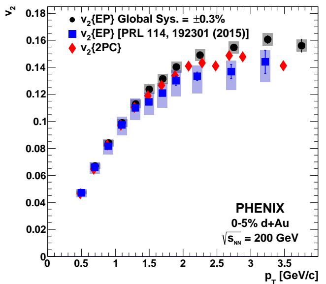
FIG. 4. The v_2 vs p_T in 0%-5% central d+Au collisions at \sqrt{s_{NN}} = 200 GeV using the event-plane method (black filled circles) and two-particle correlations (red filled diamonds). Also shown are the previously published v_2 vs p_T using the event-plane method (blue filled squares) from PHENIX using data collected in 2008 [15].
