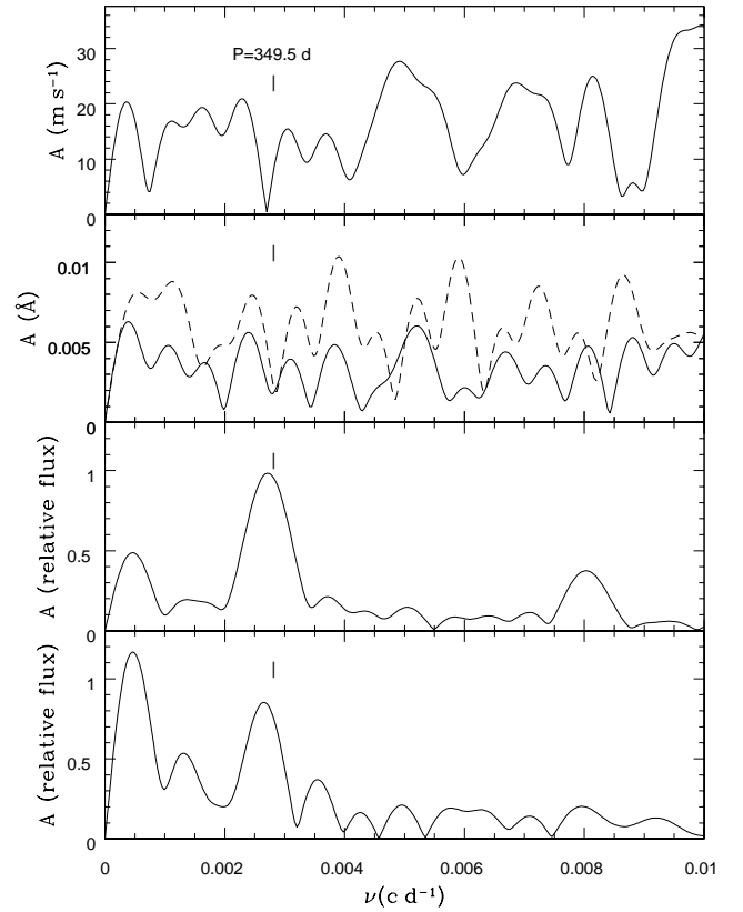
Figure 6. Top: The frequency spectrum of bisector velocity spans. Second from the top: The frequency spectrum of Ca II 8662 Å spectral line equivalent width measurements (solid line is the frequency spectrum for equivalent width measurements from 8661.0 to 8663.27 Å and dashed line from 8661.55 to 8662.8 Å). Second from the bottom: The frequency spectrum of the Kepler raw data without aligning individual quarters. Bottom: The frequency spectrum of merged Kepler data. See text for more details. A is the amplitude of the frequency spectra. The vertical line corresponds to the orbital period of the planetary candidate.
