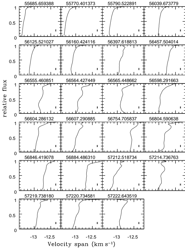
Figure 9. Spectral line bisectors for all spectra of HD 175370 observed by the HERMES spectrograph, measured from the cross-correlation function based on \sim 1650 spectral lines. BJD of the observation is shown on top of each bisector plot. Bisector velocity span errors are shown at lower right of each plot.
