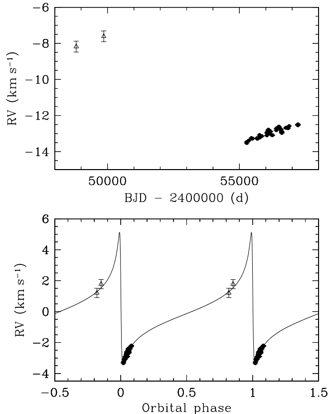
Figure 1. Top: The RV measurements of HD 175370 and their error bars from this work (filled circles) and from Famaey et al. (2005) (open triangles). Bottom: The RV measurements of HD 175370 and their error bars as above phased to the orbital period of 32,120 d with an orbital solution overlotted (solid curve).
