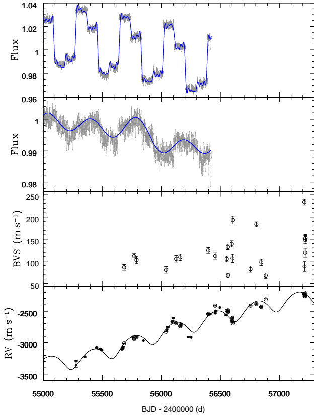
Figure 5. Top: The raw Kepler data of quarters Q2 – Q17 (grey curve). The blue curve is the sum of sine functions of periods found by PERIOD04. Second from the top: The merged Kepler light curve of quarters Q2 – Q17 (grey curve) where one can see both long-period changes and short-period changes due to stellar oscillations. The blue curve is the sum of sine functions of three long periods found by PERIOD04. Second from the bottom: Bisector velocity spans (BVS) measured from the average bisector values between flux levels of 0.1 – 0.3 and 0.7 – 0.9 of the continuum value, shown with corresponding error bars. Bottom: The RV variations of HD 175370 (TLS: filled circles, HERMES: open circles) shown for comparison.
