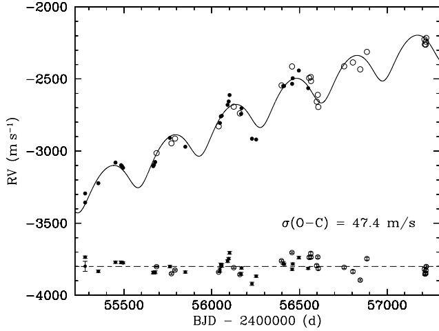
Figure 2. The RV measurements of HD 175370 obtained from March 2010 to July 2015 using the coude echelle spectrograph at TLS, Germany (filled circles) and the HERMES spectrograph at Mercator, La Palma (open circles). The solid curve is the superposition of the binary and planetary orbital solutions (see Table 4). The RV residuals and the error bars after removing the binary and planetary orbital solutions are shown in the lower part.
