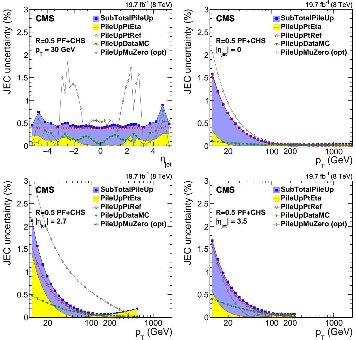
Figure 8: Pileup offset correction uncertainties for the average 2012 (8 TeV) conditions for PF jets with CHS and R = 0.5 as a function of \eta_{\text{jet}} for fixed p_{\text{T}} = 30 \text{ GeV} (top left) and as a function of jet p_{\text{T}} (top right, and bottom panels). The plots are limited to a jet energy E = p_{\text{T}} \cosh \eta = 4000 \text{ GeV} so as to show only uncertainties for reasonable p_{\text{T}} in the considered data-taking period. PileUpMuZero is an optional alternative uncertainty for zero-pileup ( \langle \mu \rangle \approx 0 ) events, and it is therefore not included in the quadratic sum SubTotalPileUp . It accounts for the pileup uncertainty absorbed in the residual response corrections at \langle \mu \rangle \approx 20 , which is particularly prominent at 1.5 < |\eta| < 3 .
