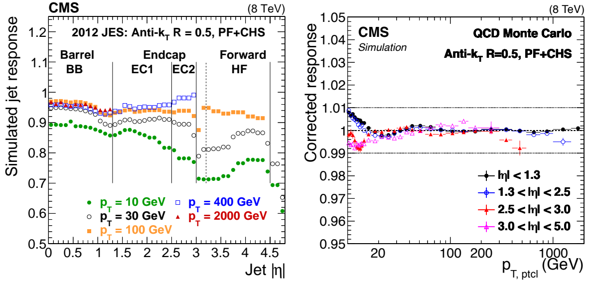
Figure 10: Simulated jet response R_{ptcl} versus |\eta| for R = 0.5 (left). Simulated jet response R_{ptcl} , after JEC have been applied, versus p_{T,ptcl} for R = 0.5 in various \eta regions, and with statistical uncertainties (right).
