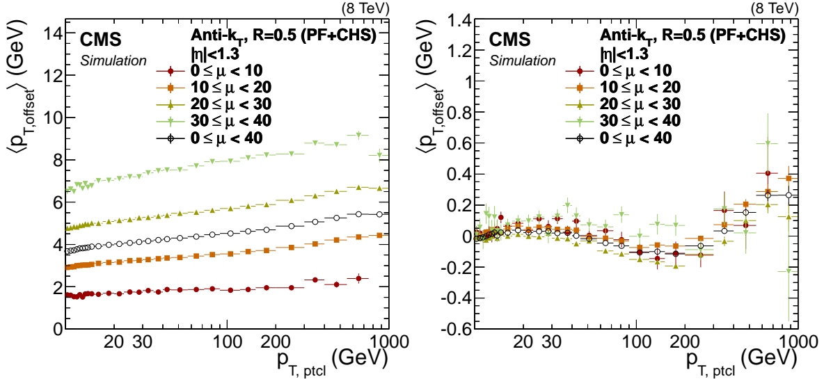
Figure 5: Simulated particle-level offset \langle p_{T, \text{offset ptcl}} \rangle defined in Eq. (3) (left), and residual offset after correcting for pileup with Eq. (2) (right) for |\eta| < 1.3 , versus particle jet p_T , for different values of average number of pileup interactions per bunch crossing \langle \mu \rangle .
