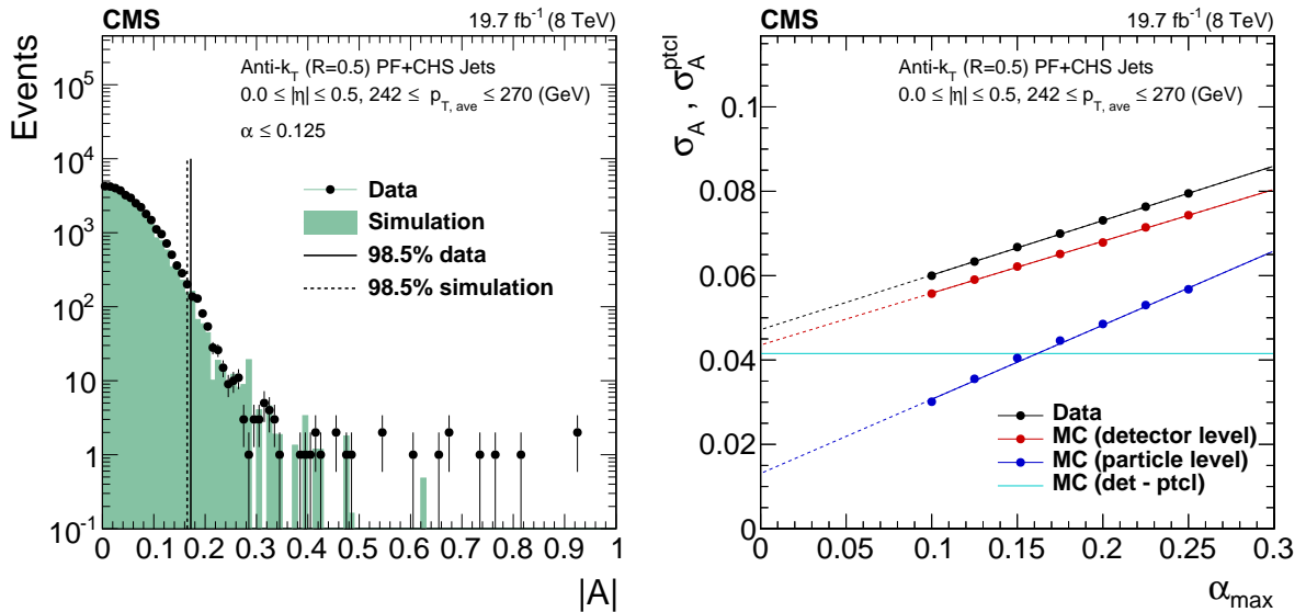
Figure 39: Left: Asymmetry distribution, Eq. (39), for data and simulation for jets with p_T \approx 250 \text{ GeV} and |\eta| < 0.5 . Right: Asymmetry measured for various thresholds \alpha_{\text{max}} , extrapolated to zero additional jet activity, for jets with p_T \approx 250 \text{ GeV} and |\eta| < 0.5 in data and MC simulation at the detector- and particle-level. The light horizontal line indicates the average particle-level resolution obtained as the difference in quadrature of MC simulation reconstructed asymmetry and particle-level imbalance, extrapolated to zero additional jet activity.
