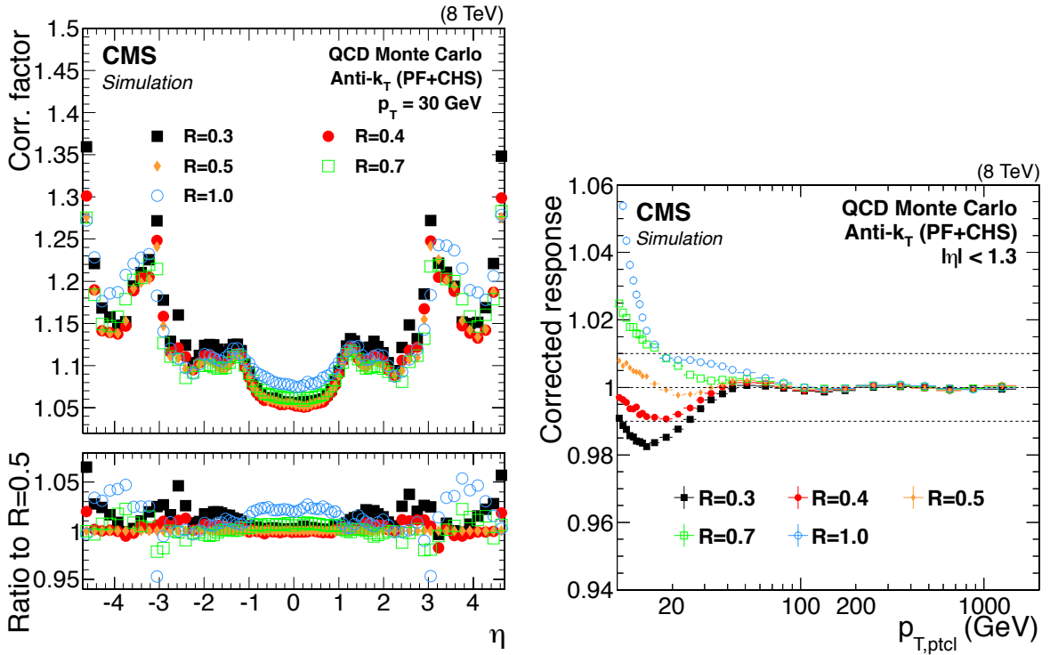
Figure 11: Jet energy correction factors for a jet with p_T = 30 GeV, as a function of \eta and for various jet sizes R (left). Simulated jet energy response R_{ptcl} after JEC for |\eta| < 1.3 as a function of the particle-level jet p_T for various jet sizes R (right).
