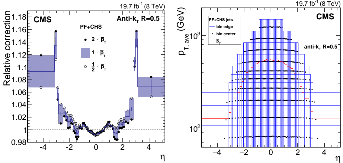
Figure 17: Relative \eta correction factor at the crossover \bar{p}_T (defined as the value of p_T where the log-linear and constant fits versus p_{T,ave} agree) value, and at half and twice the \bar{p}_T values (left). The statistical uncertainty in the constant fit at each value of \bar{p}_T is also shown. Distribution of the p_T and \eta bins used in the dijet balance measurement, with a point at the average p_T and \eta for each bin (right). The horizontal red lines indicate the crossover \bar{p}_T value for each bin.
