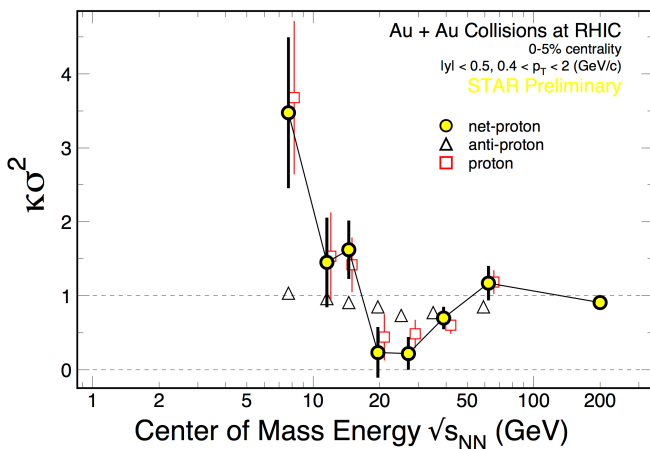
FIG. 7. Energy dependence of the product \kappa\sigma^2 (excess kurtosis times variance) of the net-proton multiplicity distribution (yellow circles) for top 0-5% central Au+Au collisions. The Poisson expectation is denoted as dotted line at \kappa\sigma^2 = 1 [50, 51].
