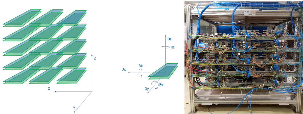
Figure 3.28: Idealised view of the cosmic ray stand with its reference frame, on the left, and a real picture of it, on the right.
