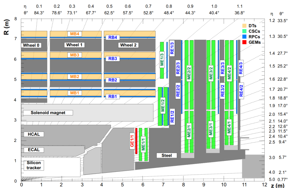
Figure 3.7: A quadrant of the R - z cross-section of the CMS detector, with the addition of the proposed GE1/1 detector (highlighted in red) within the CMS muon system [115].
