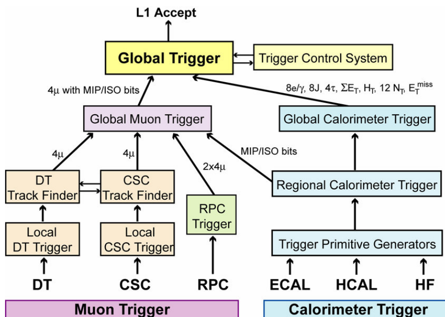
Figure 3.6: Architecture of the Level-1 Trigger.
