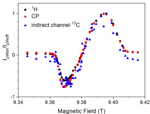
Figure 7: Normalized DNP enhancement profiles of 18 mmol kg^{-1} AMUPol in C_{10}E_6 for ^1H MAS (black squares), ^1H \rightarrow ^{13}C CP MAS DNP (red circles) and the ^{13}C MAS indirect channel resonance (blue triangles). (Taken from ref. [177]).
