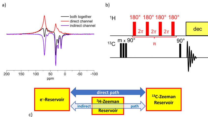
Figure 5: ^{13}\text{C} -DNP NMR: (a) DNP enhanced ^{13}\text{C} MAS NMR spectra of 20 mmol \text{kg}^{-1} AMUpol in \text{C}_{10}\text{E}_6 : spectrum recorded without additional pulses (black line), with additional 180^\circ pulses on ^1\text{H} (red line) representing the spectrum obtained via the direct channel, and difference spectrum of both, representing the spectrum obtained via the indirect channel (violet line). (b) Employed pulse sequence to suppress the indirect channel resonance (adapted from ref. [169]). (c) Cartoon of the different polarization transfer pathways.
