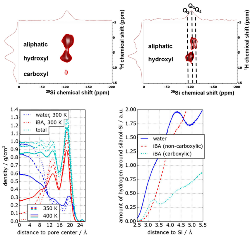
Figure 3: Upper row: 2D ^1\text{H} - ^{29}\text{Si} FSLG HETCOR of iBA/H 2 O mixtures (56 wt% iBA, 9.4 T, 110 K, 8 kHz MAS, 89 kHz FSLG homonuclear decoupling [163]) confined in SBA-15 (left: long contact time of 3 ms; right: short contact time of 0.5 ms). Lower row: MD simulations: left: density profiles for iBA and water (pore center at 0 Å; pore wall at 25 Å); right: hydrogen atom density as a function of the distance to the closest surface silanol group. The center of the pore is at 0 Å and the pore boundary is at 25 Å. (Figure adapted from Harrach et al. [162]).
