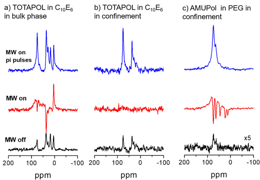
Figure 8: Comparison of ^{13}\text{C} MAS spectra obtained for (a) 15 mM TOTAPOL in \text{C}_{10}\text{E}_6 bulk phase, (b) 15 mM TOTAPOL in \text{C}_{10}\text{E}_6 in SBA-APTES confinement, and (c) 15 mM AMUPol in PEG 200 in SBA-APTES confinement. Spectra were recorded with MW on and MW off. Additional MW on spectra were recorded employing the sequence displayed in Figure 5(b), which suppresses indirect channel resonances (see Hoffmann et al. [164] for details).
