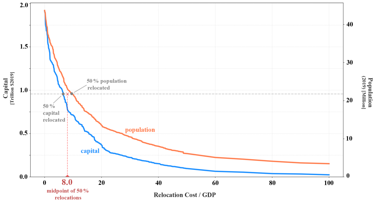
Figure 2. Calibration of the non-market relocation cost parameter based on the revealed preference of current populations. Curves show the magnitude of the population (orange) and physical capital (blue) that is instantaneously relocated in the optimal adaptation scenario of pyCIAM, assuming SSP2–IIASA socioeconomic projections and median no-climate change RSLR, as a function of this parameter. The parameter is normalized by local GDP per capita. We identify the parameter values for which 50% of the population and capital instantaneously relocated under an assumption of zero non-market costs are no longer relocated and average these two values to estimate the relocation parameter used in pyCIAM.
