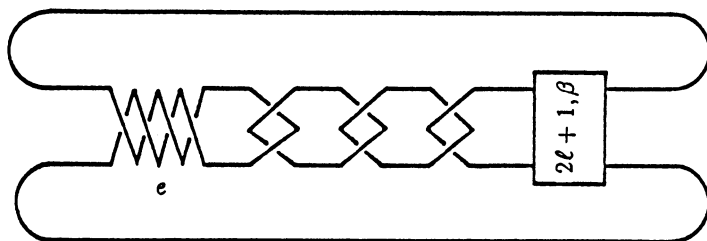
Montesinos link m(0; e_0; 1/2, 1/2, 1/2, \beta/2\ell + 1) , e = e_0 + 3/2 + \beta/2\ell + 1 \in \mathbb{Z}
