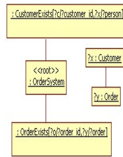
Figure 13. The placeOrder(?c) post-condition
