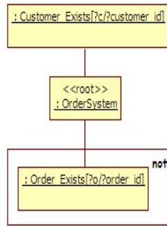
Figure 12. The placeOrder(?c) pre-condition
