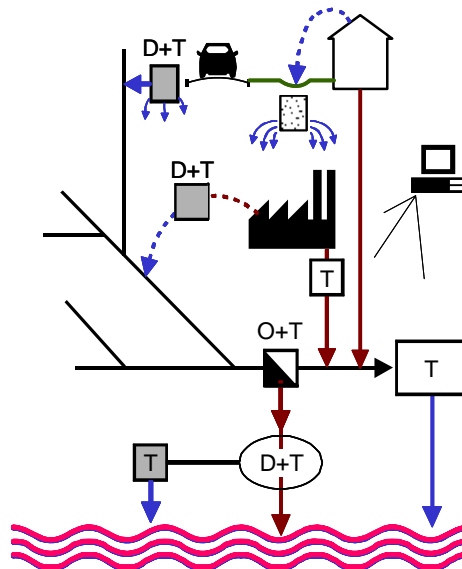
Fig. 1. Representation of the physical system considered in the ScorePP project, exemplified with a combined sewer system including both upstream (source control) and downstream (end-of-pipe treatment) mitigation options. In addition to the shown point discharges (treatment plants and combined sewer overflows) there are diffuse discharges from e.g. building drains and unknown pipe networks and overland flow. D: Detention, O: Overflow, T: Treatment.
