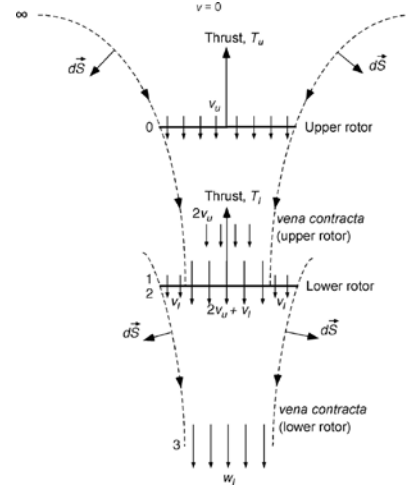
Figure 3 - Model of a Co-Axial Rotor System [8].
