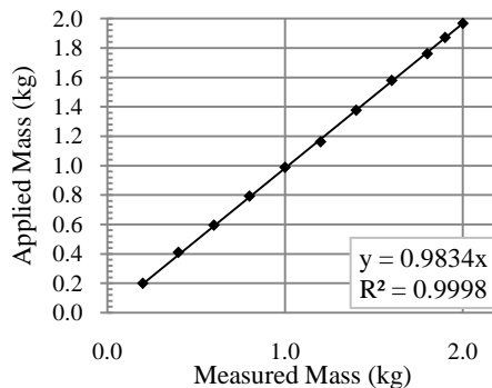
Figure 6 - Fine Test Rig Calibration Results.
