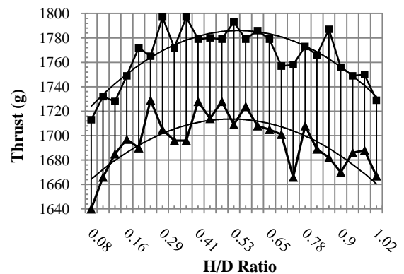
Figure 7 - Variation of Co-Axial Thrust with Rotor Spacing.
