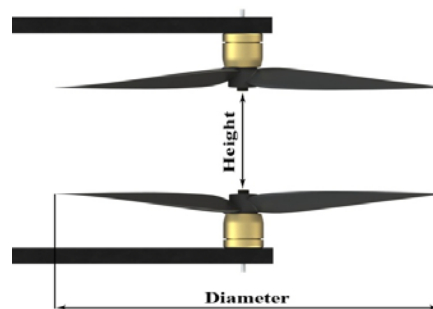
Figure 4 – Inter-Rotor Separation Distance.
