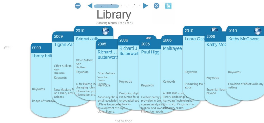
Figure 1: INVISQUE Interface
