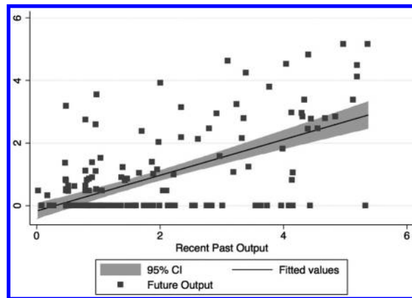
FIGURE 1.—A SCATTER PLOT OF FUTURE OUTPUT AND RECENT PAST OUTPUT
