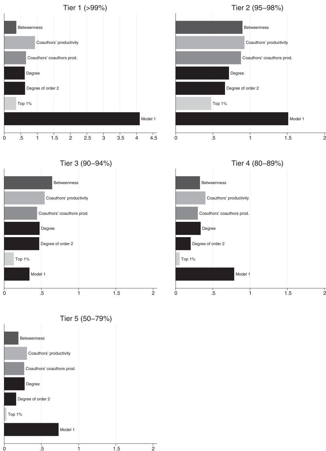
FIGURE 7.—RMSE % DIFFERENCE BETWEEN RESTRICTED MODELS ACROSS PRODUCTIVITY TIERS
