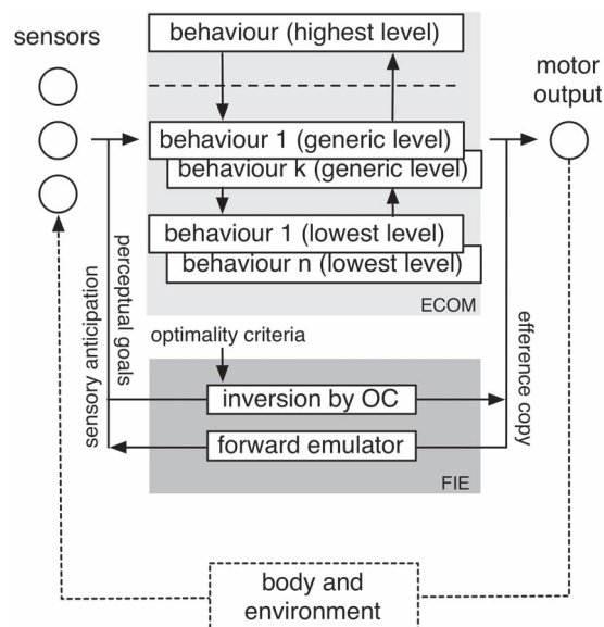
Fig. 4. Architecture of the co-driver for the CRF implementation of the Continuous Support function.
