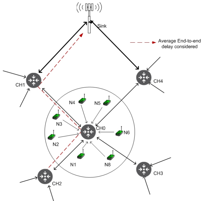
Figure 1: Network topology of the reference scenario
