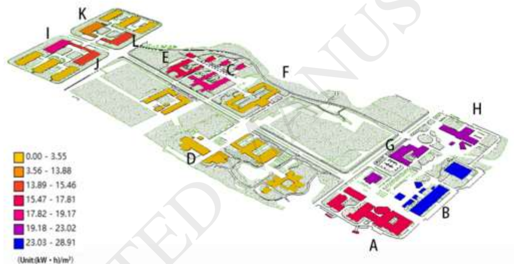
Fig. 5. Seasonal electricity consumption intensity of space heating in campus buildings in winter.
