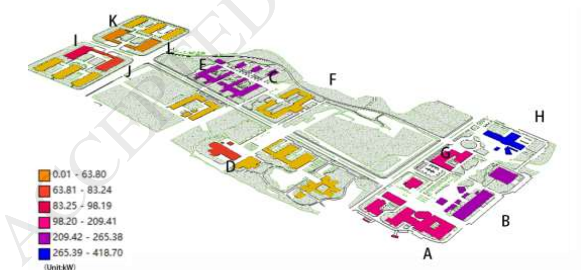
Fig. 3. Daily peak load of space heating in campus buildings in winter.
