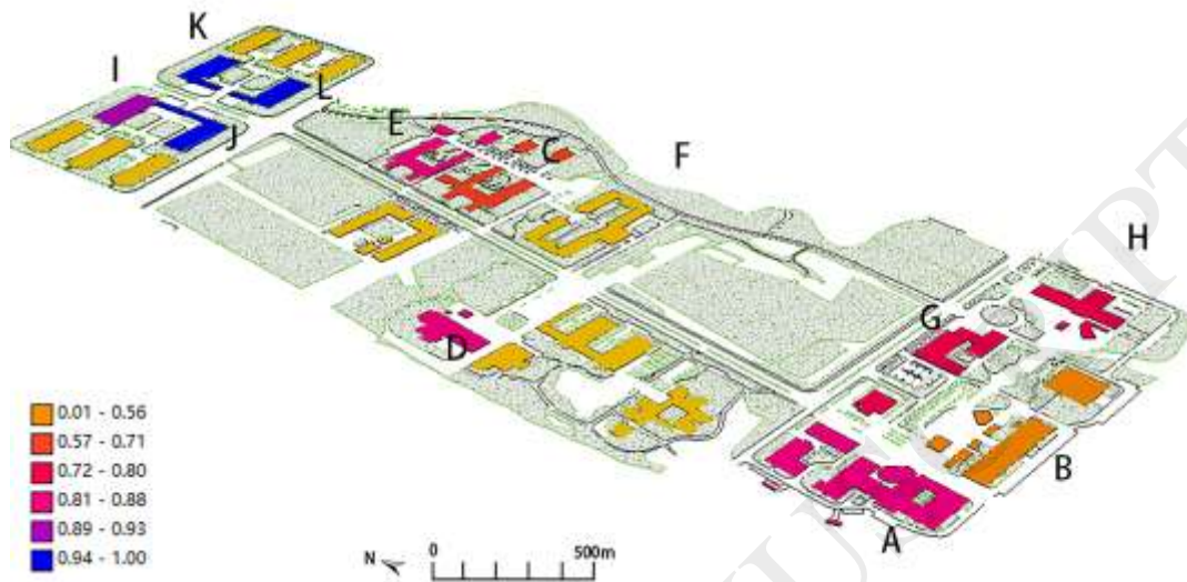
Fig. 6. Daily peak-to-valley difference ratio of space heating in campus buildings in winter.
