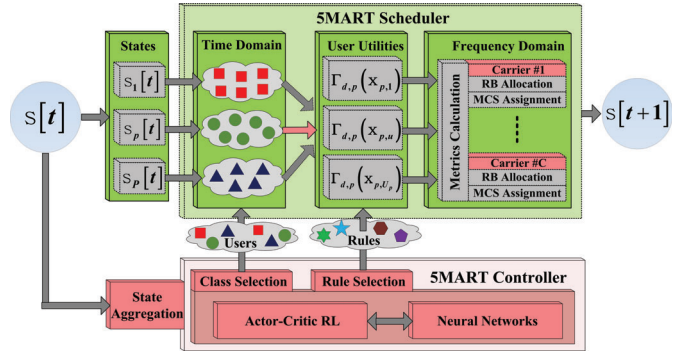
Fig. 1. Proposed SMART framework.
