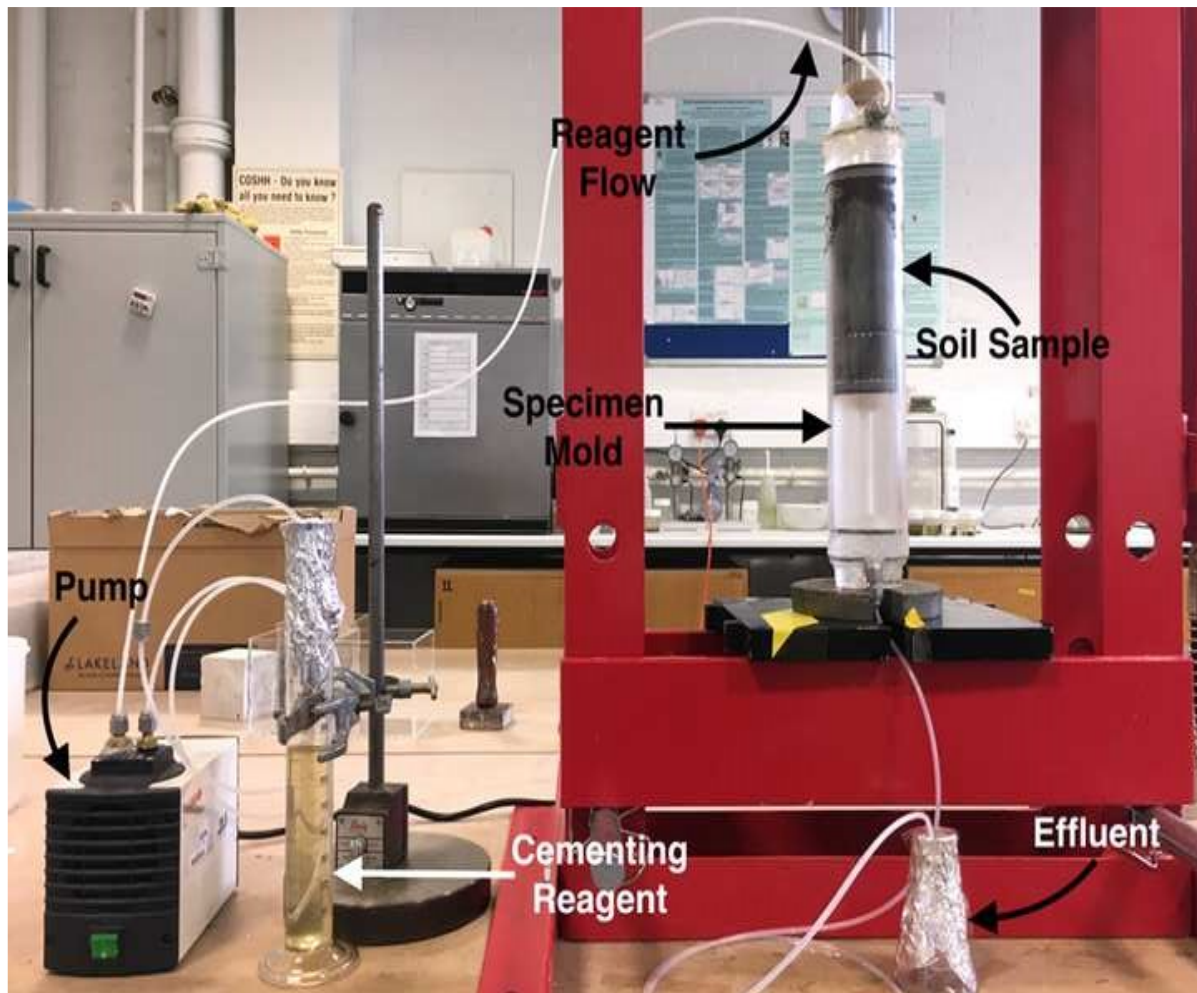
Fig. 2. Pressure flow column set up
