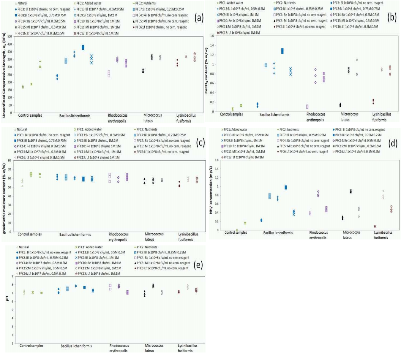
Fig 4. Pressure flow column results: (a) unconfined compressive strength, q_u (kPa); (b) \text{CaCO}_3 content (% w/w) (end of test); (c) Moisture content (% w/w of dry soil) (end of test); (d) maximum \text{NH}_4^+ concentration (mg/L); (e) end-of-test pH
