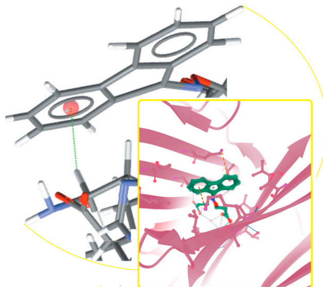
Figure 4. Bio-complex showing the C-H... \pi Fmoc interaction (PDB code 3gs4) [131].
