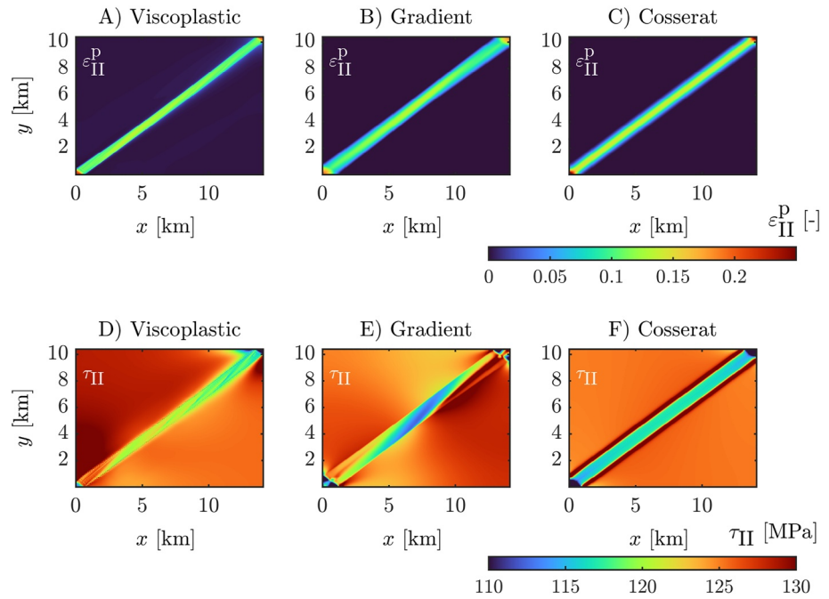
Figure 2. Shear banding pattern obtained with the various regularizations after 40 time steps ( t = 1.1 Kyr). The upper row correspond to accumulated plastic strain and the lower row depicts the second invariant of the deviatoric stress tensor. Viscoplasticity (A, D, \eta^p = 10^{18} Pa · s), gradient plasticity (B, E, K_g = 5 \times 10^{12} Pa · m 2 ) and the use of a Cosserat continuum (C, F, l_c = 80 m).
