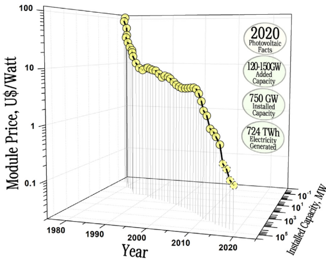
Fig. 2. Photovoltaic module price slide and 2020 photovoltaic facts. The values of historic module price are informative rather than exact since data are retrieved from LaFond's diagram where sources beyond 2016 are extrapolated [11].
