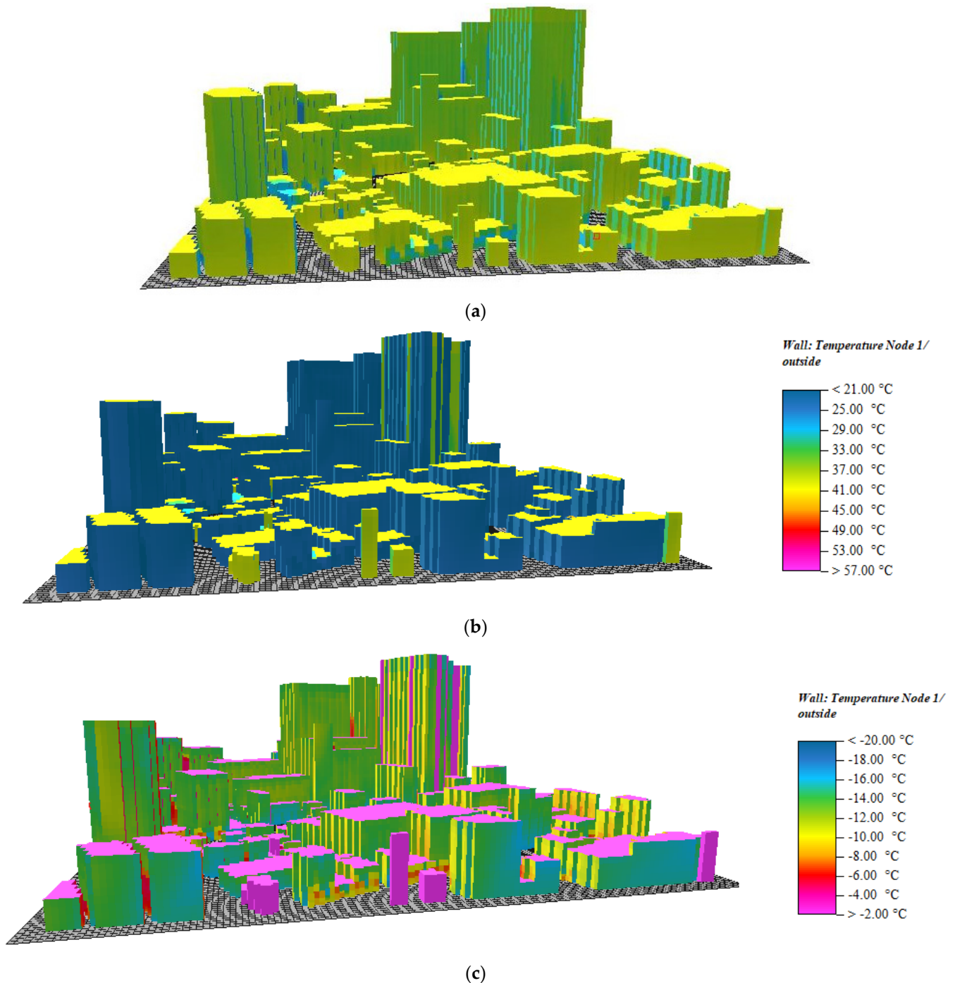
Figure 11. Walls temperature; (a) Scenario A, (b) Scenario E, (c) the difference between Scenarios A and E.
