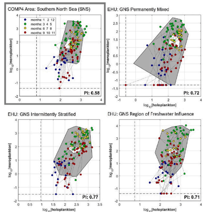
Fig. 7. Plankton Index lifeform-lifeform plots for the regions shown in Fig. 5: ‘Southern North Sea’ (SNS) COMP4 area (upper left, emphasised by grey box) and the three EHUs which partially overlap SNS. Circles, coloured by season, are paired holoplankton-meroplankton abundances (logarithmic scale) during the ‘comparison period’ (2006–2015), overlain on the ‘assessment envelope’ defined by each region’s ‘assessed period’ data (grey doughnut shape, monthly data not shown). The PI values (bottom right of each plot) are the ratio of the number of points which fall inside to that which fall outside of the assessment envelopes.
