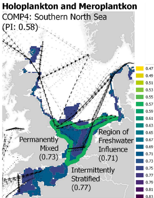
Fig. 6. PI and spatial extent comparison between the Southern North Sea COMP4 area and overlapping ecohydrodynamic units. PI values for the holoplankton & meroplankton lifeform pair are given in brackets and shown in the same colour scale as in Fig. 4. The Southern North Sea COMP4 area is designated with a thick (green) outline. EHD units are coloured by their PI values in dark blues (Permanently Mixed, dotted black outline; Region of Freshwater Influence, dashed outline) and mid-blue (Intermittently stratified). Black semi-transparent dashed and dotted lines show CPR survey tracks since 2000, with darker lines indication overlapping sampling over time. (For interpretation of the references to colour in this figure legend, the reader is referred to the web version of this article.)
