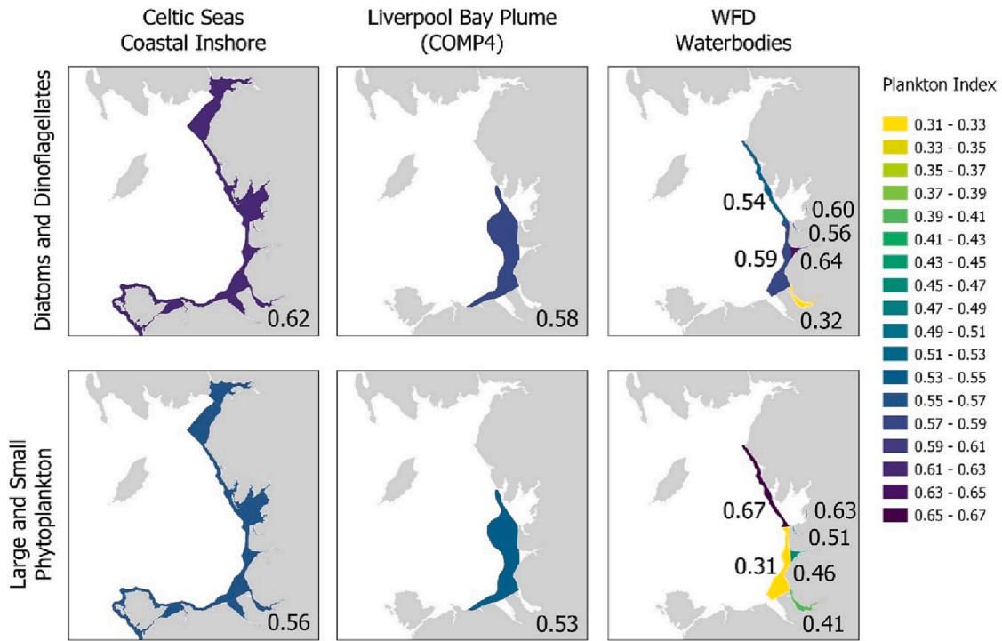
Fig. 8. PI values derived from Environment Agency monitoring data at different spatial scales. using monthly averages of: (left) all data in OSPAR Region II: Celtic Seas; (Centre) all data in in the Liverpool Bay Plume COMP4 area, and (right) all available data in each of the WFD Transitional and Coastal waterbodies. WFD waterbodies without sufficient monitoring to derive high confidence PIs for the chosen time period are not shown, though observations from these areas are included in the larger spatial aggregations. Upper row shows PI values for the diatoms & dinoflagellates lifeform pair, lower row for large & small phytoplankton.
