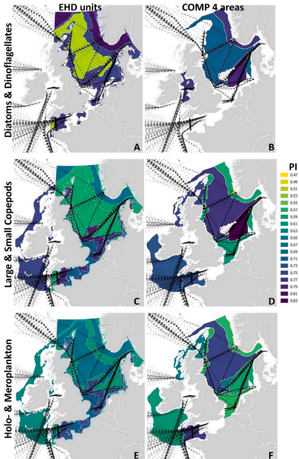
Fig. 4. PI values derived from CPR data, with darker colours indicating no or small changes in plankton community structure and lighter and brighter colours indicating larger changes. A,C,E for ecohydrodynamic units divided east–west into OSPAR Regions II and III, and B,D,F for COMP4 assessment areas. Areas within OSPAR Regions II and III with insufficient data to derive high-confidence PI values are in white. Black dashed and dotted lines show CPR survey tracks since 2000.
