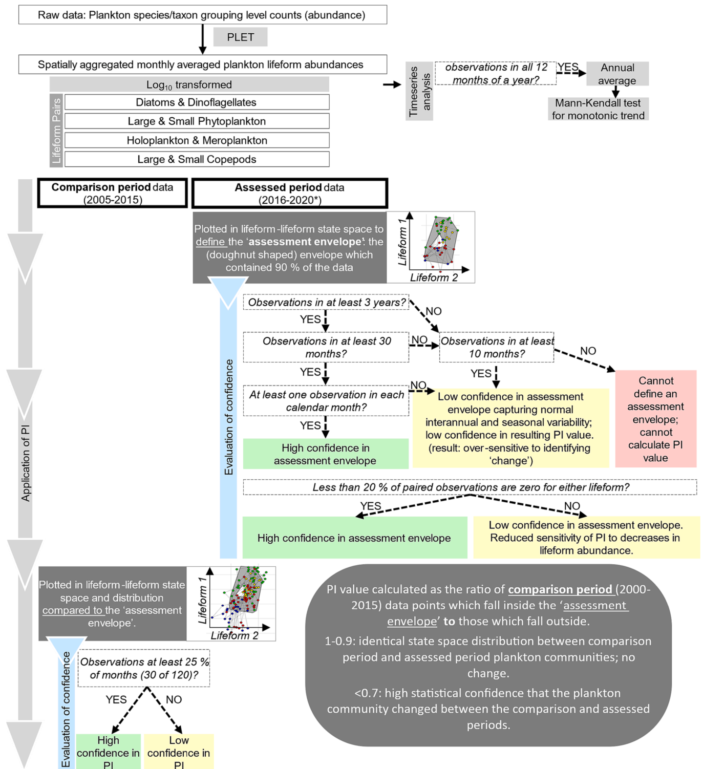
Fig. 3. Schematic representation of Plankton Index (PI) calculation workflow, including criteria for evaluating confidence in resulting PI based on availability of monthly monitoring data throughout both the comparison and assessed periods of the timeseries. PLET: the Plankton Lifeform Extraction tool (PLET; Ostle et al., 2021). See Supplemental Methods for more details.
