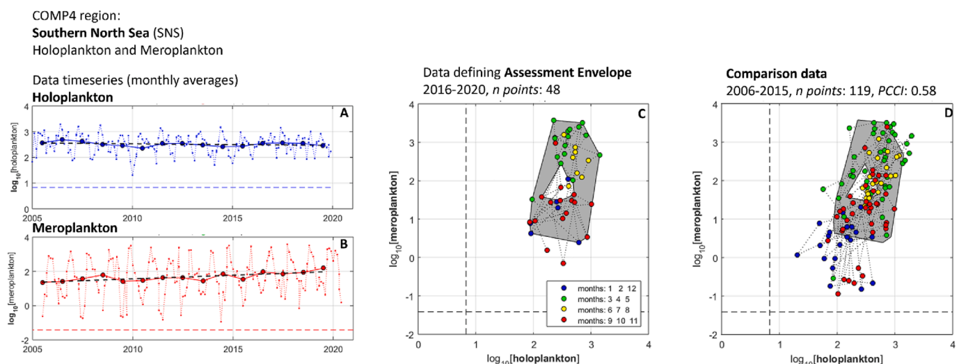
Fig. 5. CPR lifeform abundances for the holoplankton and meroplankton lifeform pair derived for the Southern North Sea (SNS) COMP4 area. A & B: timeseries of lifeform abundances showing monthly average abundances (small coloured points, where dashed coloured lines join observations from consecutive months) and annual average values (large circles with black borders, connected by solid line) with linear fit (dashed black line) to annual averages (significant increase in meroplankton, Mann-Kendall p = 0.0004 ; no trend in holoplankton, Mann-Kendall p = 0.3 ). C: paired observations during the assessed period (circles, coloured by season), and resulting assessment envelope (grey doughnut shape), D: paired observations during the comparison period, overlain on the assessment envelope from C.
