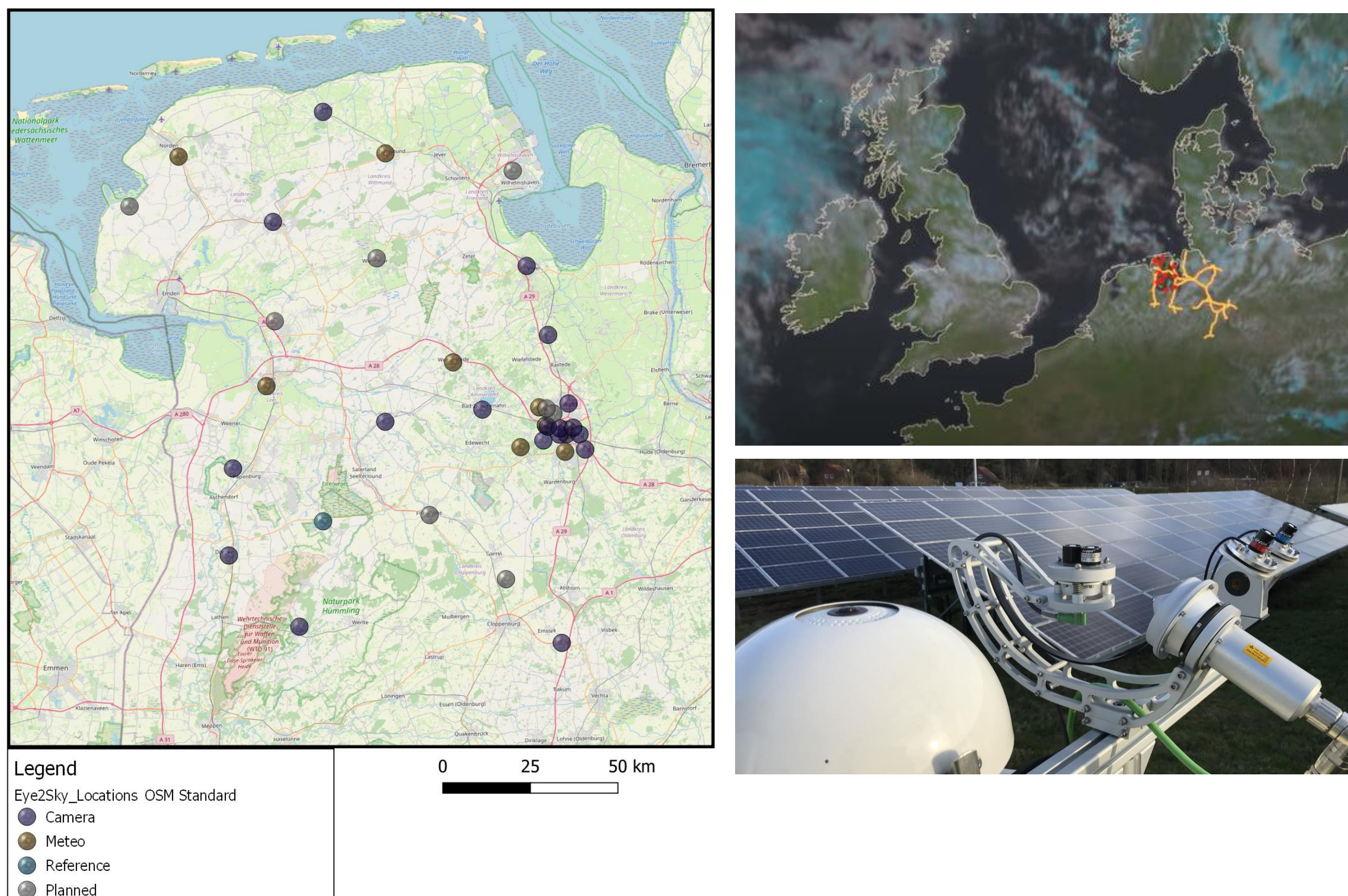
Fig. 1: Map of the Eye2Sky network (left), illustration of a satellite view of the area (top right) and the instrumentation of a station with meteorological sensors showing the camera, the rotating shadowband irradiometer and the sensors for irradiance on a tilted plane (bottom right).
