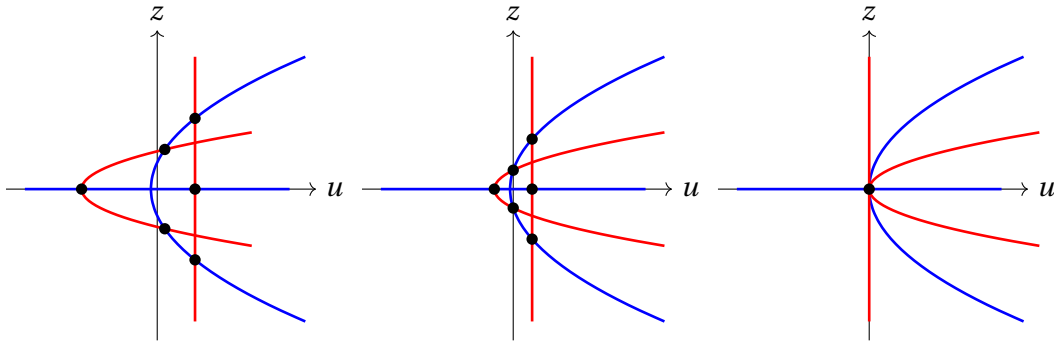
Figure 5.1: Graphical representation of the points associated to the family of radical ideals \{I_3(t)\}_{t \in \mathbb{C}} , defined in Example 5.1.7, with t \rightarrow 0 . The red graphic represents the polynomial h_{3,1}(t) , and the blue one represents the polynomial h_{3,0}(t) .
