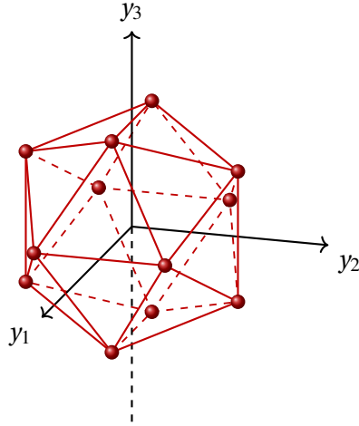
Figure 3.2: Graphical representation of decomposition (3.3.6), whose elements correspond, up to central simmetry, to the vertices of a regular icosahedron.
