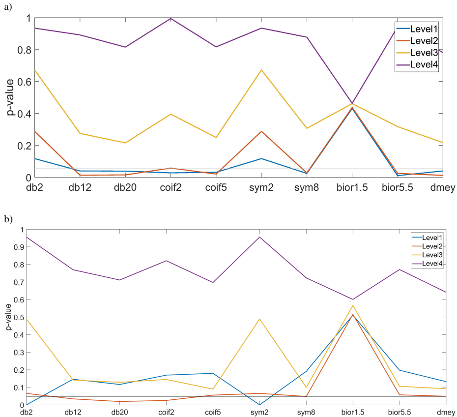
Fig. 4. p-value for the lowest increment angle with respect to the building platform, a) Dq parameter b) Da parameter. Grey horizontal line indicates the critical value.
