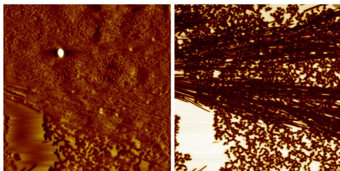
Figure 2. (left) 6.6 \times 6.6 \mu\text{m}^2 AFM topography scan of the droplet-prepared sample with its (right) corresponding phase image (z-height scale \approx 70 nm and phase voltage scale \approx 5.2 V).
