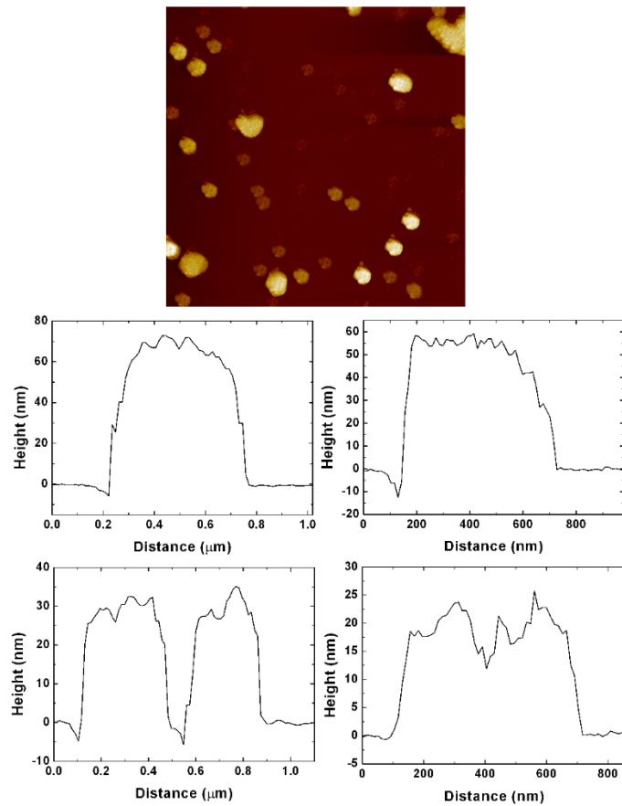
Figure 3. (top) 6.6 \times 6.6 \mu\text{m}^2 AFM topography scan of the 1 h dip-coated sample (z-height scale \approx 80 \text{ nm} ) with (bottom) representative height profiles of several colloidal clusters showing their relative height to the surrounding surface.
