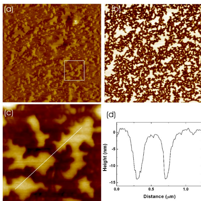
Figure 1. (a) 6.6 \times 6.6 \mu\text{m}^2 AFM topography scan of the droplet-prepared sample (z-height scale \approx 50 nm) with (b) associated phase image (voltage range 4.87 V) and (c) magnified section with (d) height profile.
