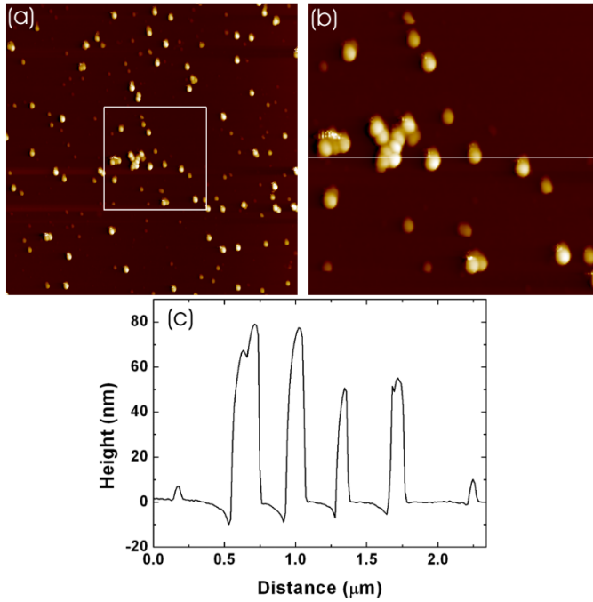
Figure 7. (a) 6.6 \times 6.6 \mu\text{m}^2 AFM topography scan of the sample submersed for 240 h in the suspension (z-height scale \approx 80 nm). (b) zoom section and (c) corresponding height profile (indicated by white line on image).
