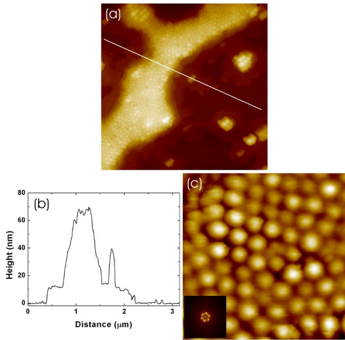
Figure 6. (a) 3 \times 3 \mu\text{m}^2 AFM topography scan (z-height scale \approx 100 nm); (b) height profile (indicated by white line on image) showing a relative height of approx. 70 nm for the of the large structure, approx. 40 nm for a small isolated cluster and a surrounding plateau layer of height approx. 12 nm. (c) Zoom of larger structure (imaged sharpened) showing hexagonal crystalline structuring of the particles along with (insert) its 2D FFT.
