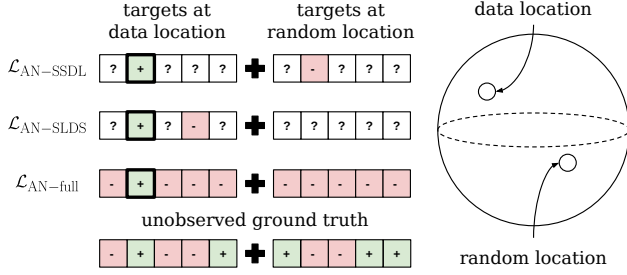
Figure 2. Illustration of the data used by three loss functions from Section 3.2. For each loss, we visualize the targets that the network is trained to predict. Each loss can be broken into two parts: one part that updates the network’s predictions at the location of a training example ( data location ) and one part that updates the network’s predictions at another location chosen randomly ( random location ). Each loss has access to one confirmed positive label (bold boxes). The rest of the labels are unobserved (non-bold boxes), and the losses make different, imperfect, assumptions about those unobserved labels.
