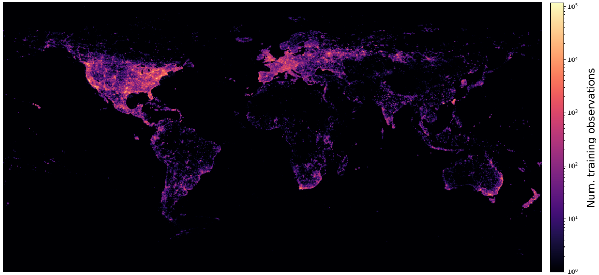
Figure A4. Histogram of the locations of the observations from our iNaturalist training set. Here we bin the data for all 35 million observations across all 47,375 species. Darker colors indicate fewer observations, brighter colors indicate more. The training data is biased towards North America, Europe, and New Zealand.
