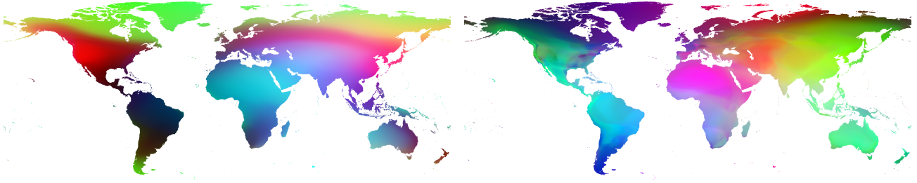
Figure 3. Visualization of the 256-dimensional features from learned location encoders f_\theta projected to three dimensions using Independent Component Analysis (ICA). All models use the \mathcal{L}_{AN-\text{full}} loss and take coordinates as input. (Left) This corresponds to a SINR model trained with a maximum of 10 examples per class. The features are smooth and do not appear to encode much high frequency spatial information. (Right) In contrast, the SINR model trained with a maximum of 1000 examples per class contains more high frequency information. The increase in training data appears to enable this model to better encode spatially varying environmental properties. Note, ICA is performed independently per-model, so similar colors do not indicate correspondence between the two images.
